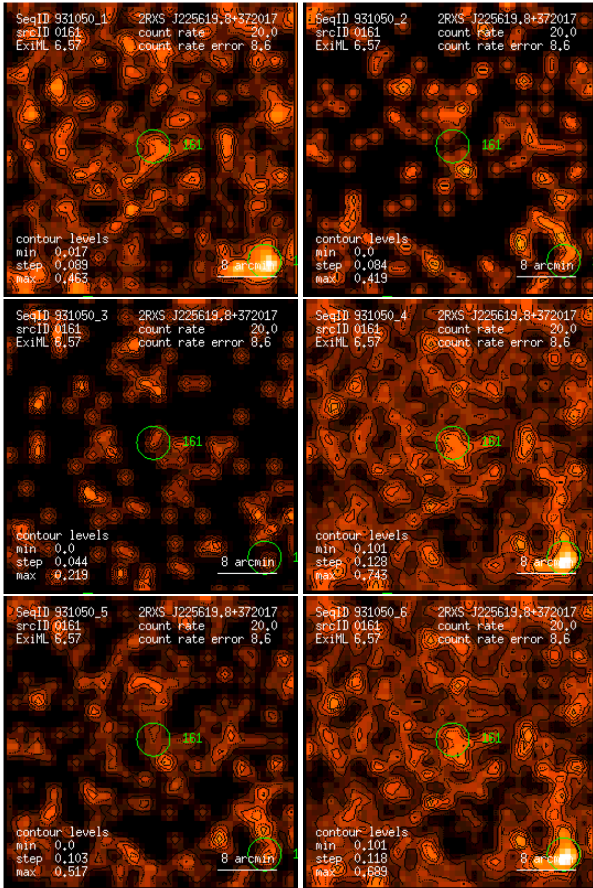
Figure 161: RASS 931050: detection 0161: band rate images, Gaussian filter: (1) PSPC channels 11 – 41, (2) 52 – 90, (3) 91 – 201, (4) 11 – 235, (5) 52 – 201, (6) 11 – 201. Broad band rates in counts/ks. Band rate contour levels in counts/ks/arcmin 2 .
