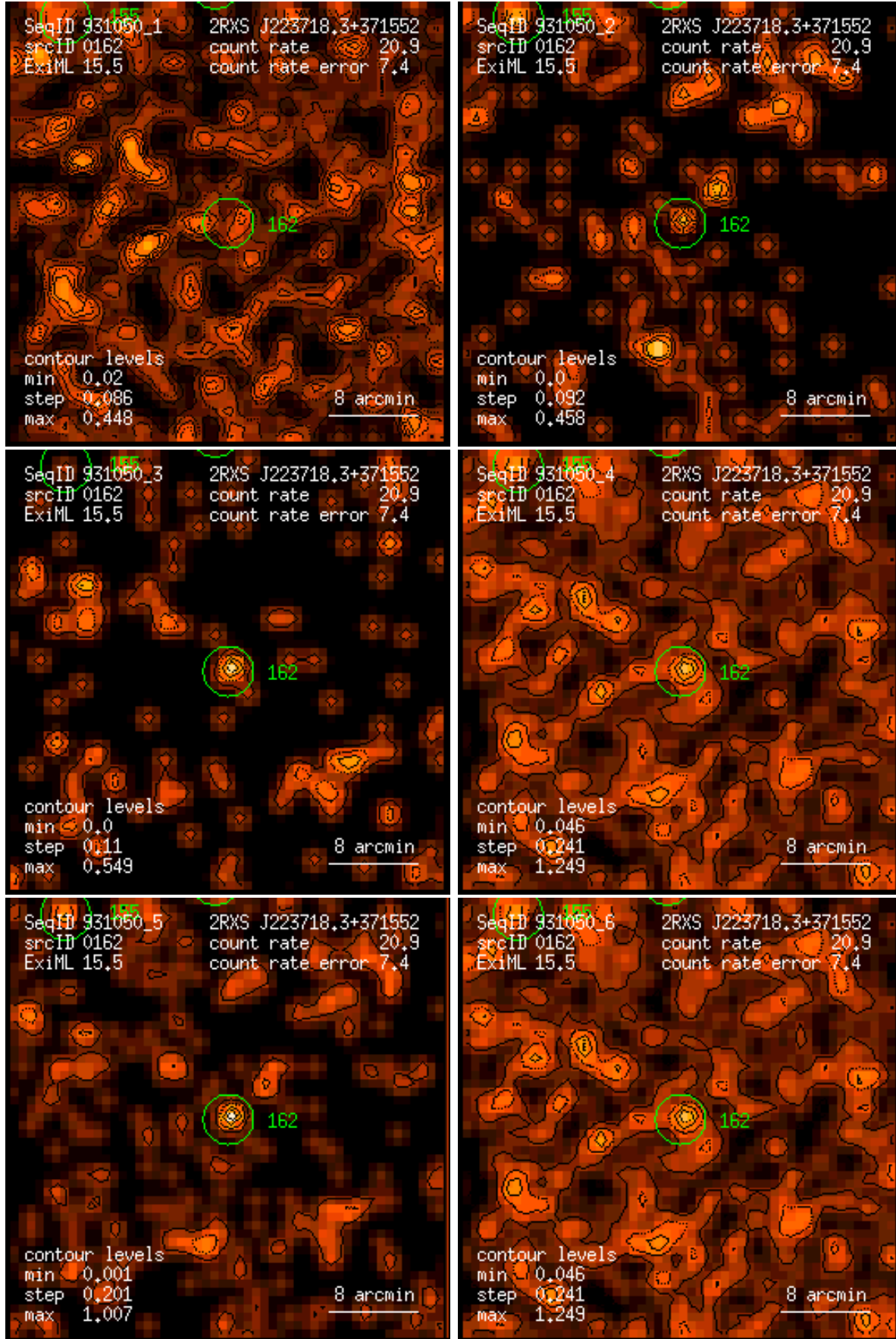
Figure 162: RASS 931050: detection 0162: band rate images, Gaussian filter: (1) PSPC channels 11 – 41, (2) 52 – 90, (3) 91 – 201, (4) 11 – 235, (5) 52 – 201, (6) 11 – 201. Broad band rates in counts/ks. Band rate contour levels in counts/ks/arcmin 2 .
