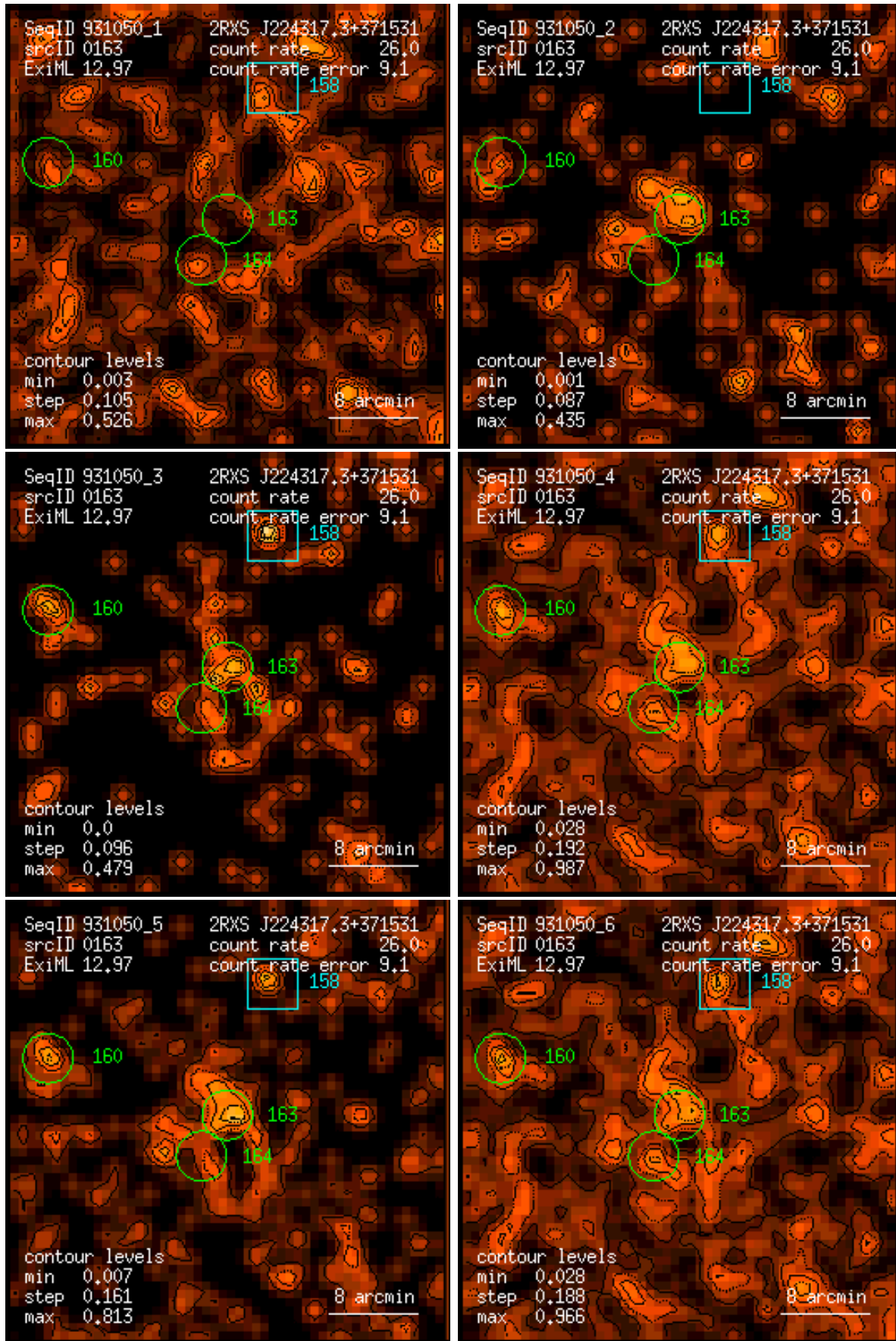
Figure 163: RASS 931050: detection 0163: band rate images, Gaussian filter: (1) PSPC channels 11 – 41, (2) 52 – 90, (3) 91 – 201, (4) 11 – 235, (5) 52 – 201, (6) 11 – 201. Broad band rates in counts/ks. Band rate contour levels in counts/ks/arcmin 2 .
