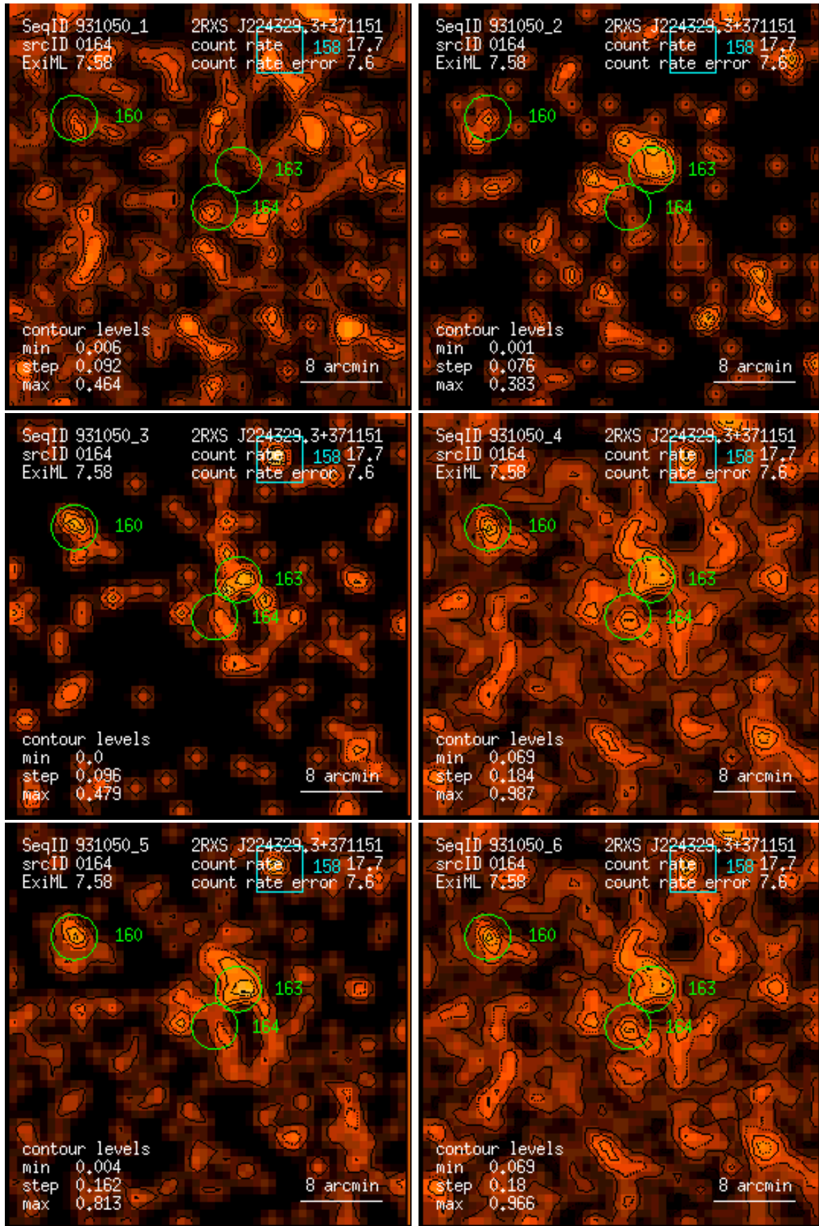
Figure 164: RASS 931050: detection 0164: band rate images, Gaussian filter: (1) PSPC channels 11 – 41, (2) 52 – 90, (3) 91 – 201, (4) 11 – 235, (5) 52 – 201, (6) 11 – 201. Broad band rates in counts/ks. Band rate contour levels in counts/ks/arcmin 2 .
