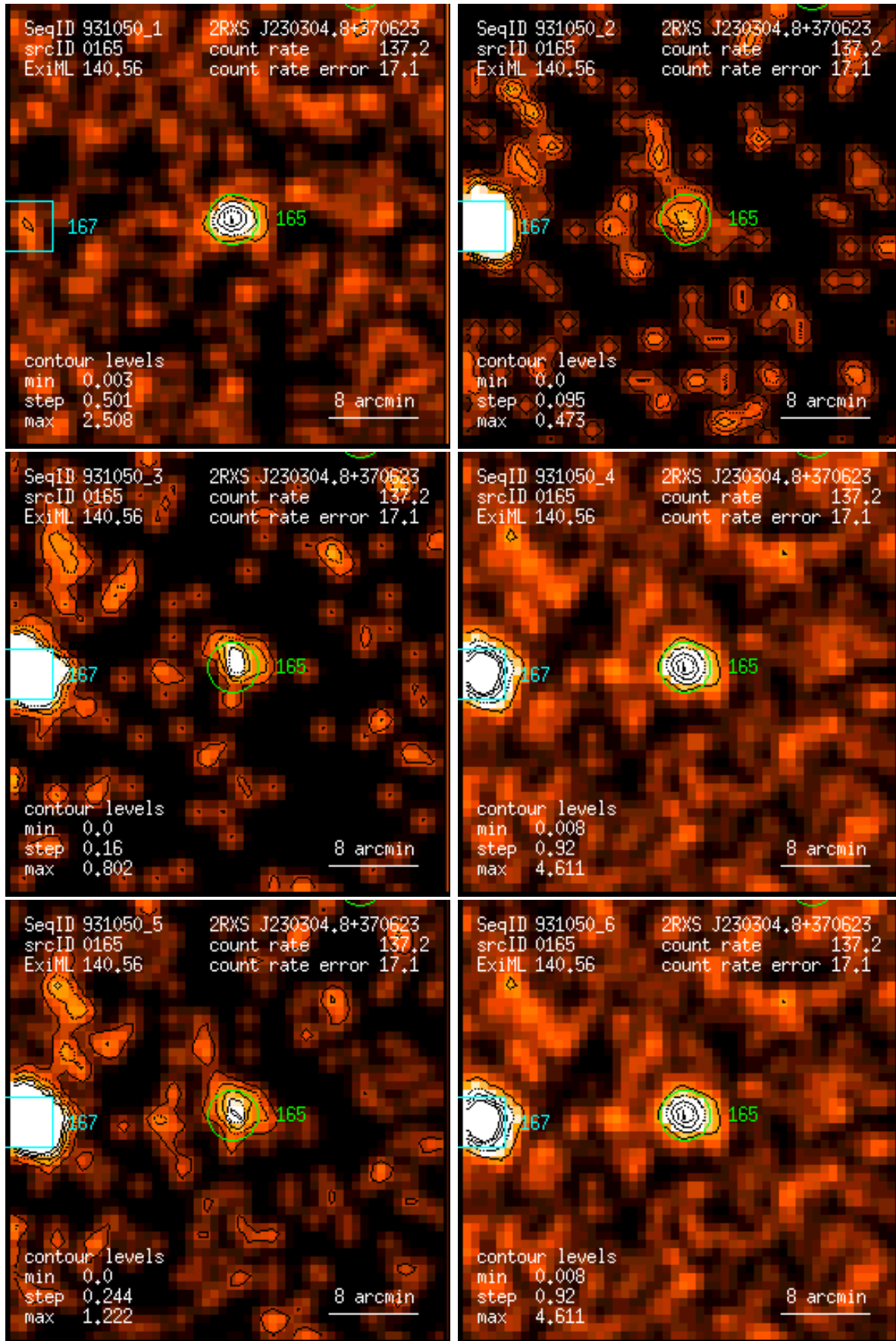
Figure 165: RASS 931050: detection 0165: band rate images, Gaussian filter: (1) PSPC channels 11 – 41, (2) 52 – 90, (3) 91 – 201, (4) 11 – 235, (5) 52 – 201, (6) 11 – 201. Broad band rates in counts/ks. Band rate contour levels in counts/ks/arcmin 2 .
