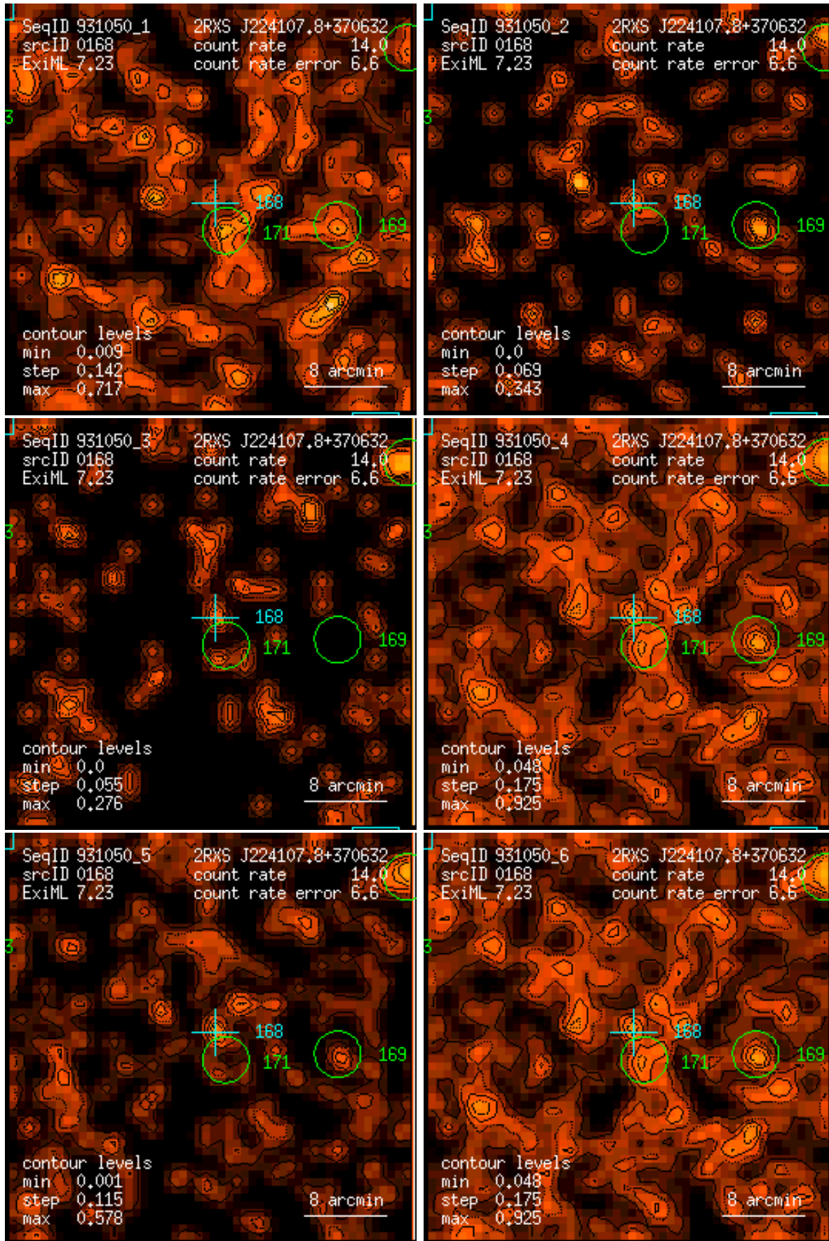
Figure 168: RASS 931050: detection 0168: band rate images, Gaussian filter: (1) PSPC channels 11 – 41, (2) 52 – 90, (3) 91 – 201, (4) 11 – 235, (5) 52 – 201, (6) 11 – 201. Broad band rates in counts/ks. Band rate contour levels in counts/ks/arcmin 2 .
