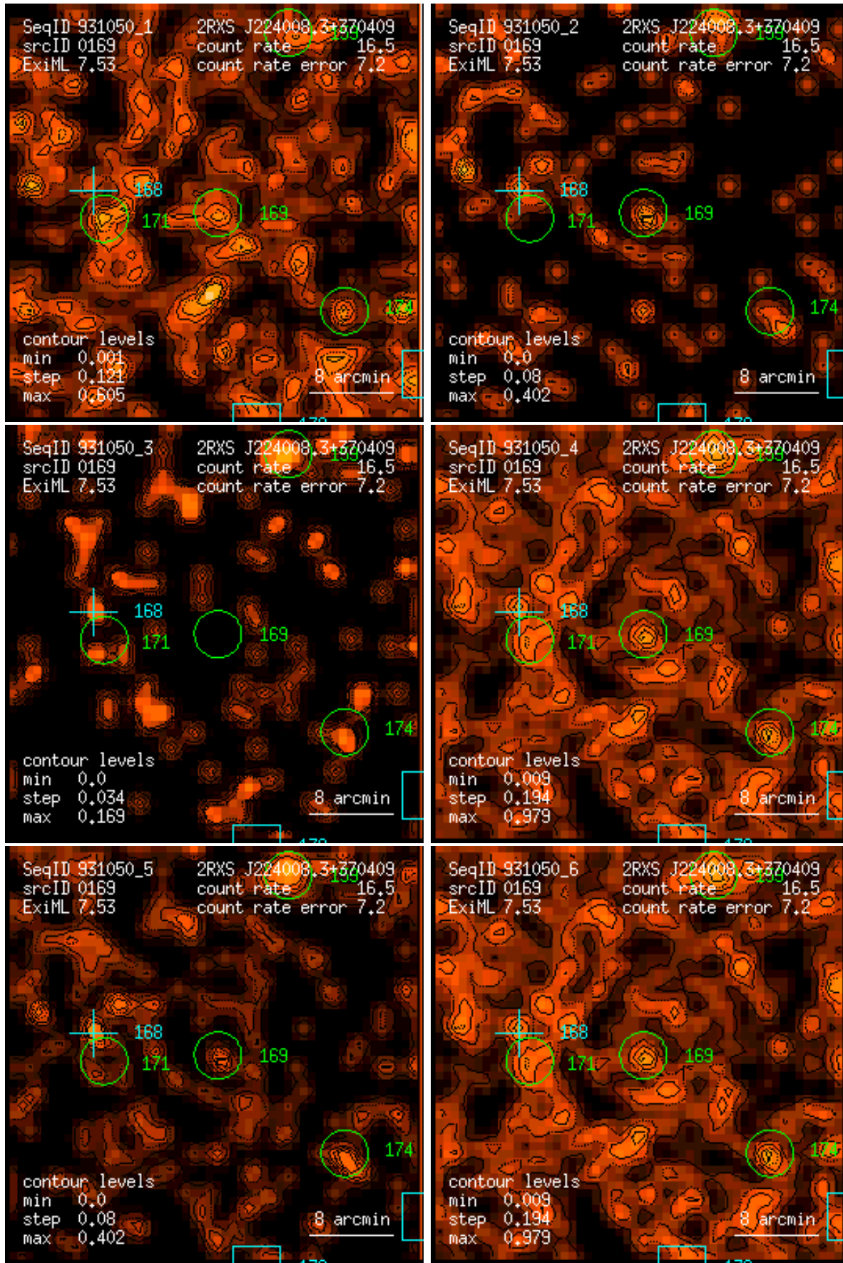
Figure 169: RASS 931050: detection 0169: band rate images, Gaussian filter: (1) PSPC channels 11 – 41, (2) 52 – 90, (3) 91 – 201, (4) 11 – 235, (5) 52 – 201, (6) 11 – 201. Broad band rates in counts/ks. Band rate contour levels in counts/ks/arcmin 2 .
