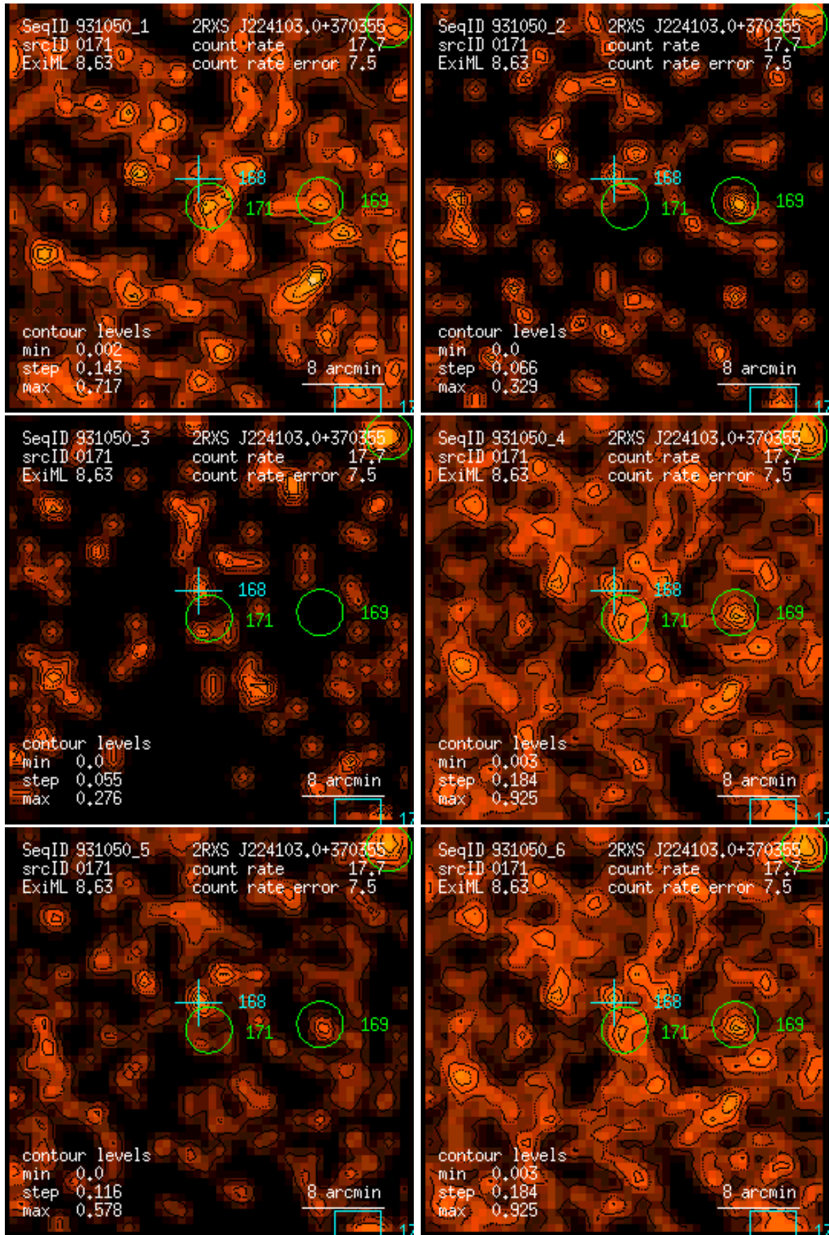
Figure 171: RASS 931050: detection 0171: band rate images, Gaussian filter: (1) PSPC channels 11 – 41, (2) 52 – 90, (3) 91 – 201, (4) 11 – 235, (5) 52 – 201, (6) 11 – 201. Broad band rates in counts/ks. Band rate contour levels in counts/ks/arcmin 2 .
