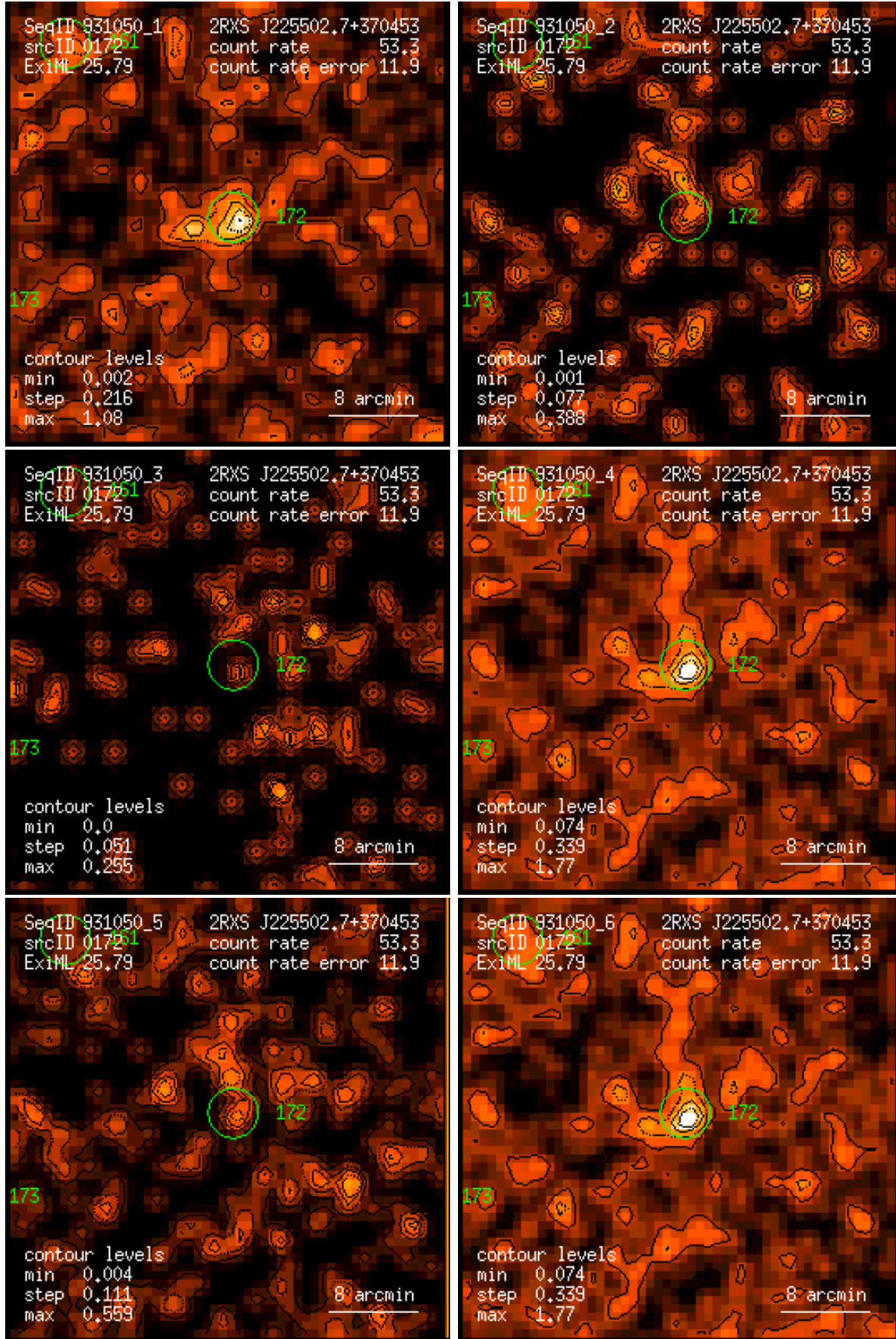
Figure 172: RASS 931050: detection 0172: band rate images, Gaussian filter: (1) PSPC channels 11 – 41, (2) 52 – 90, (3) 91 – 201, (4) 11 – 235, (5) 52 – 201, (6) 11 – 201. Broad band rates in counts/ks. Band rate contour levels in counts/ks/arcmin 2 .
