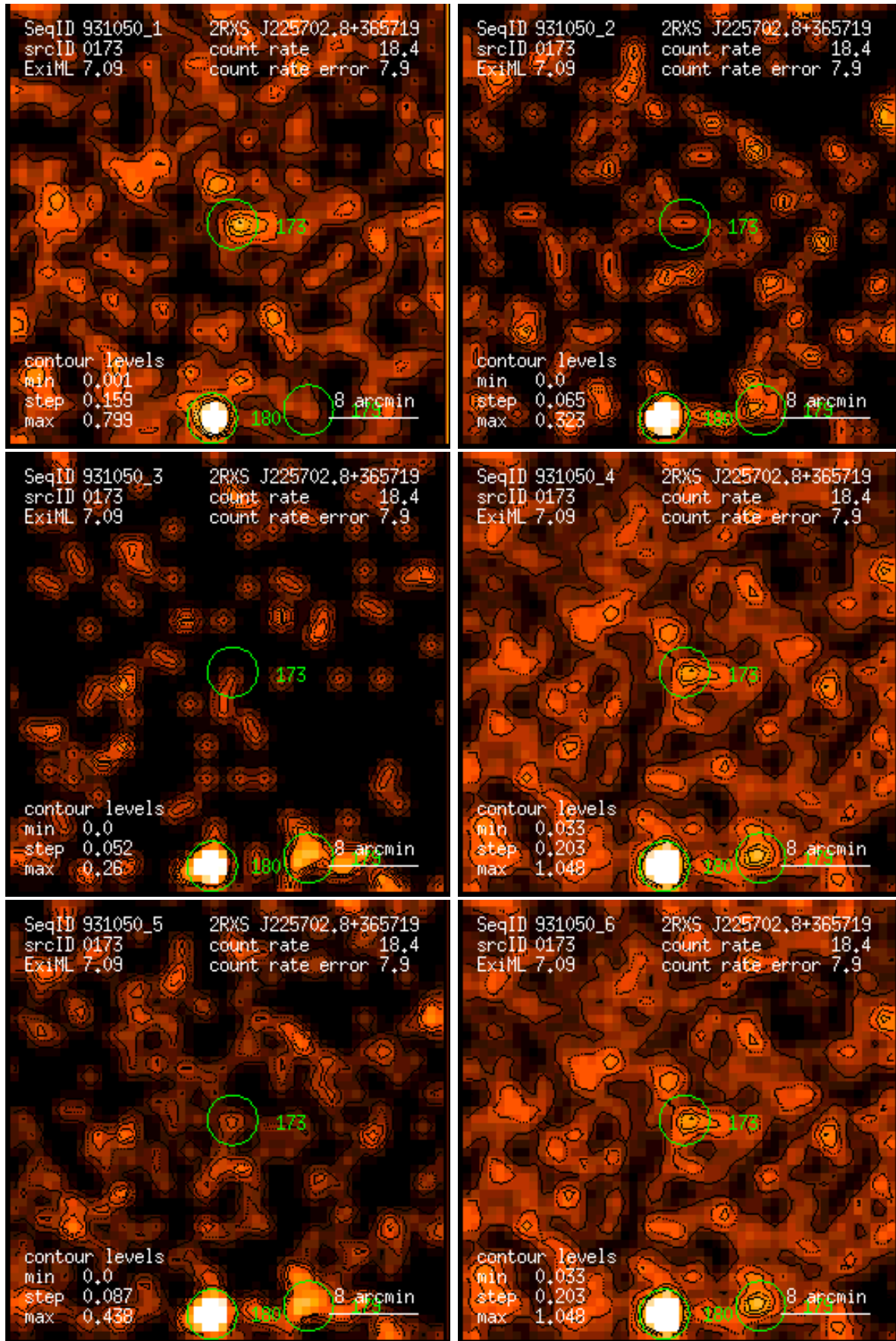
Figure 173: RASS 931050: detection 0173: band rate images, Gaussian filter: (1) PSPC channels 11 – 41, (2) 52 – 90, (3) 91 – 201, (4) 11 – 235, (5) 52 – 201, (6) 11 – 201. Broad band rates in counts/ks. Band rate contour levels in counts/ks/arcmin 2 .
