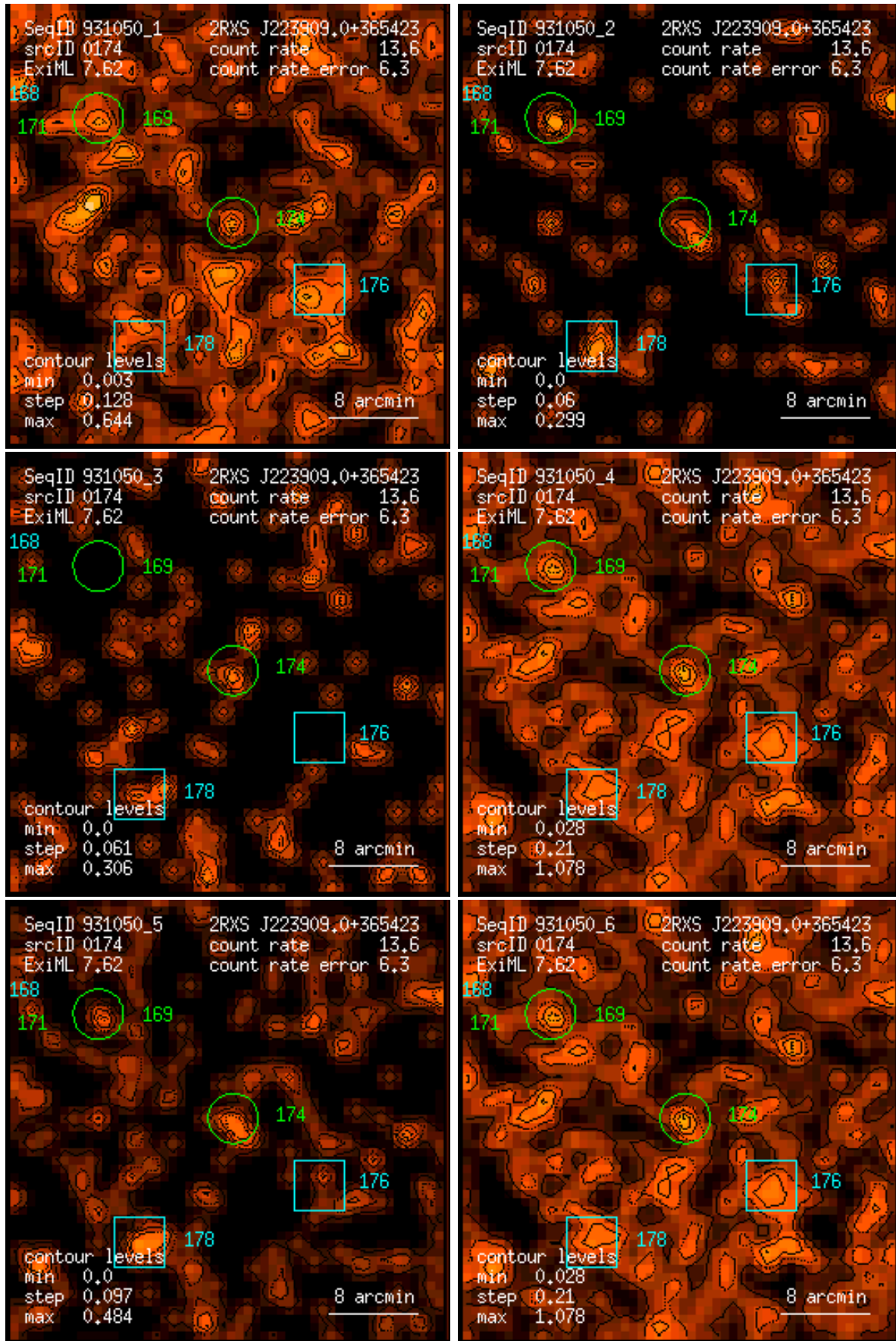
Figure 174: RASS 931050: detection 0174: band rate images, Gaussian filter: (1) PSPC channels 11 – 41, (2) 52 – 90, (3) 91 – 201, (4) 11 – 235, (5) 52 – 201, (6) 11 – 201. Broad band rates in counts/ks. Band rate contour levels in counts/ks/arcmin 2 .
