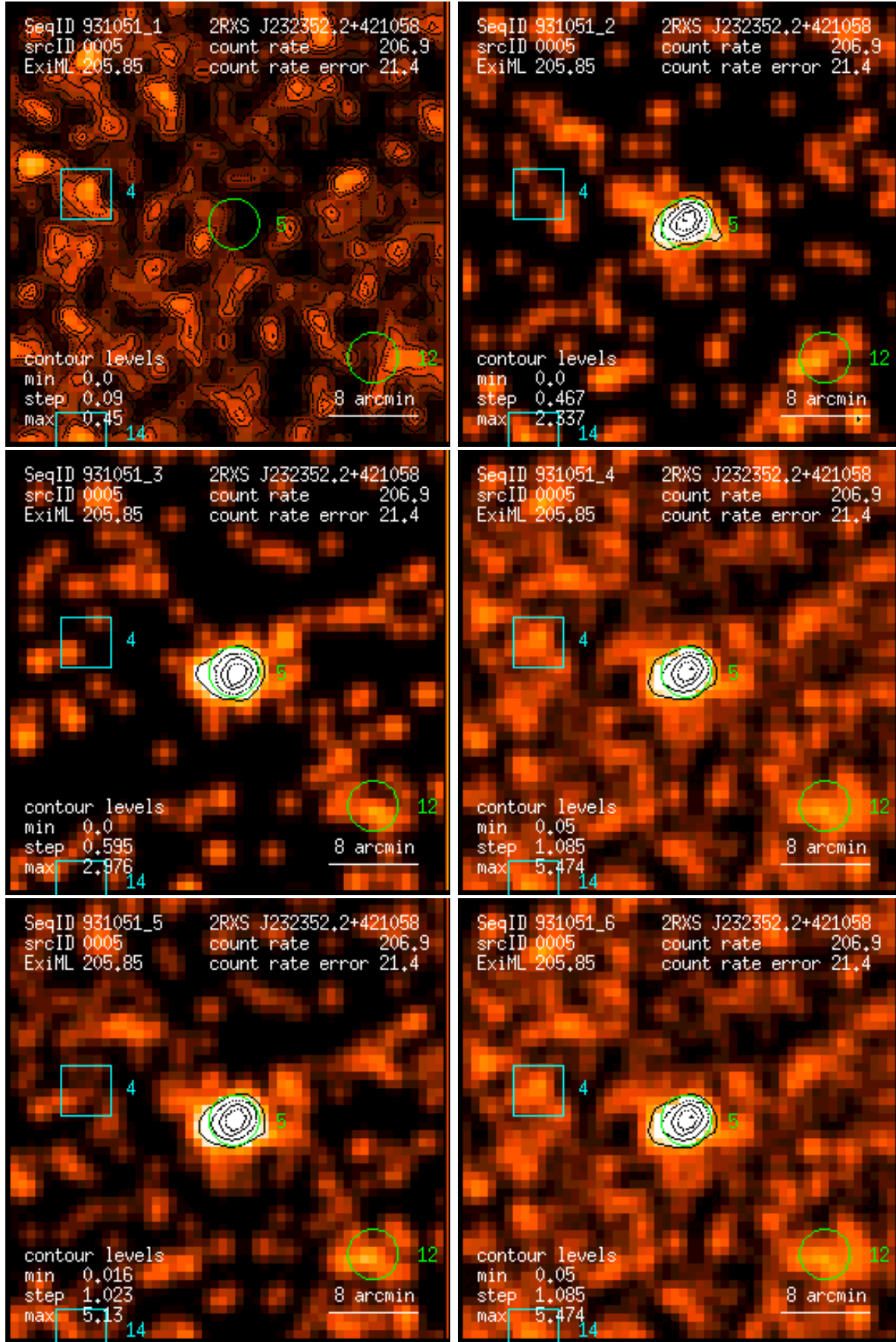
Figure 5: RASS 931051: detection 0005: band rate images, Gaussian filter: (1) PSPC channels 11 – 41, (2) 52 – 90, (3) 91 – 201, (4) 11 – 235, (5) 52 – 201, (6) 11 – 201. Broad band rates in counts/ks. Band rate contour levels in counts/ks/arcmin 2 .
