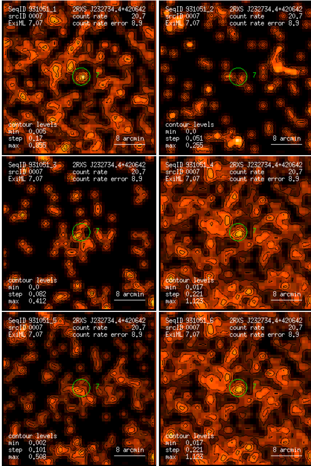
Figure 7: RASS 931051: detection 0007: band rate images, Gaussian filter: (1) PSPC channels 11 – 41, (2) 52 – 90, (3) 91 – 201, (4) 11 – 235, (5) 52 – 201, (6) 11 – 201. Broad band rates in counts/ks. Band rate contour levels in counts/ks/arcmin 2 .
