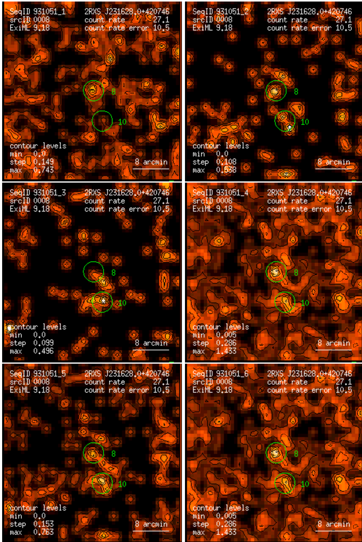
Figure 8: RASS 931051: detection 0008: band rate images, Gaussian filter: (1) PSPC channels 11 – 41, (2) 52 – 90, (3) 91 – 201, (4) 11 – 235, (5) 52 – 201, (6) 11 – 201. Broad band rates in counts/ks. Band rate contour levels in counts/ks/arcmin 2 .
