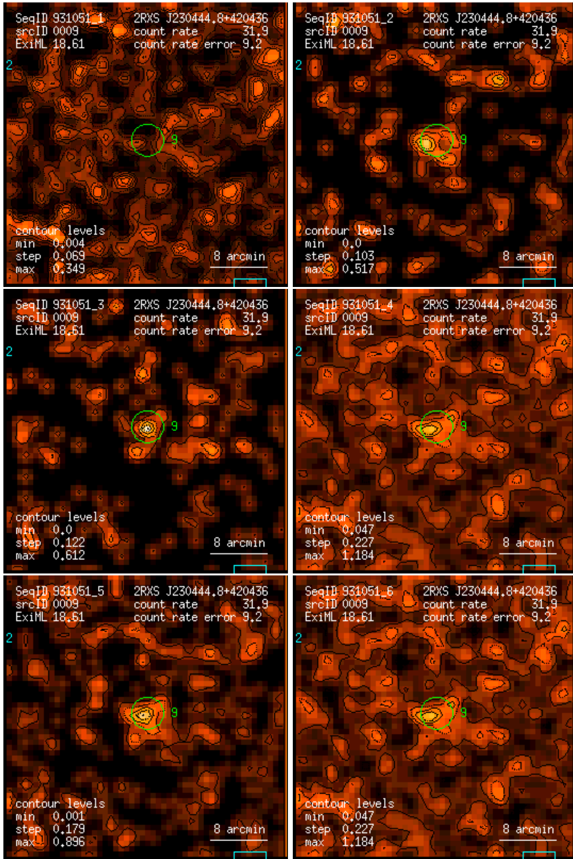
Figure 9: RASS 931051: detection 0009: band rate images, Gaussian filter: (1) PSPC channels 11 – 41, (2) 52 – 90, (3) 91 – 201, (4) 11 – 235, (5) 52 – 201, (6) 11 – 201. Broad band rates in counts/ks. Band rate contour levels in counts/ks/arcmin 2 .
