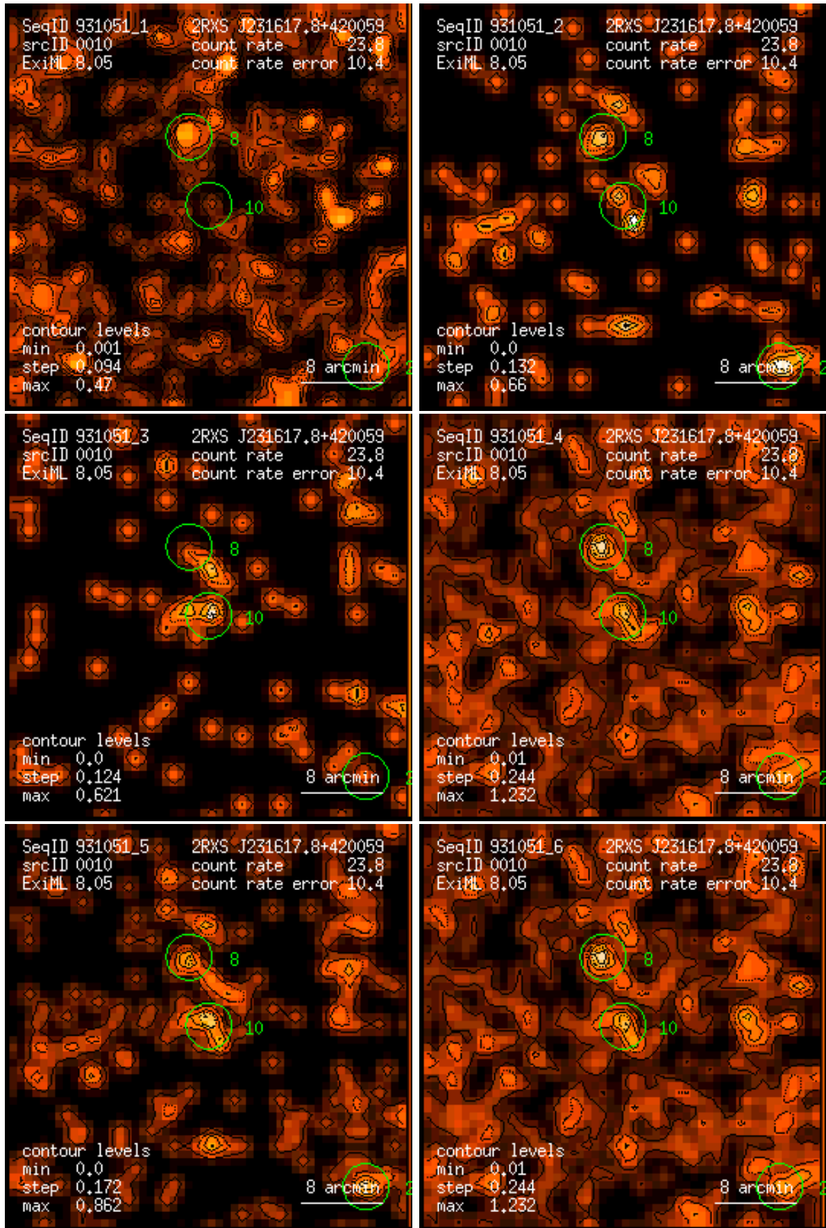
Figure 10: RASS 931051: detection 0010: band rate images, Gaussian filter: (1) PSPC channels 11 – 41, (2) 52 – 90, (3) 91 – 201, (4) 11 – 235, (5) 52 – 201, (6) 11 – 201. Broad band rates in counts/ks. Band rate contour levels in counts/ks/arcmin 2 .
