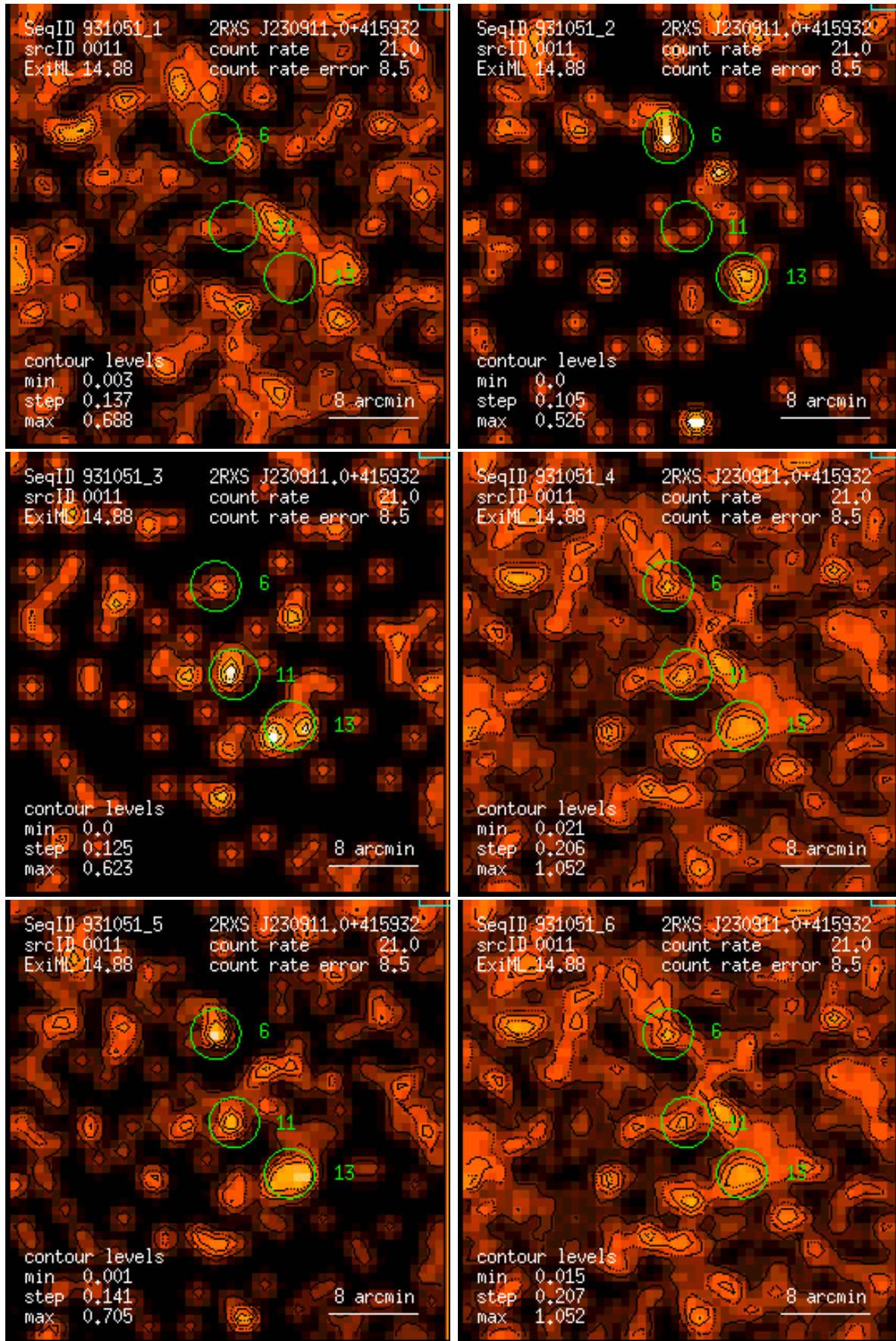
Figure 11: RASS 931051: detection 0011: band rate images, Gaussian filter: (1) PSPC channels 11 – 41, (2) 52 – 90, (3) 91 – 201, (4) 11 – 235, (5) 52 – 201, (6) 11 – 201. Broad band rates in counts/ks. Band rate contour levels in counts/ks/arcmin 2 .
