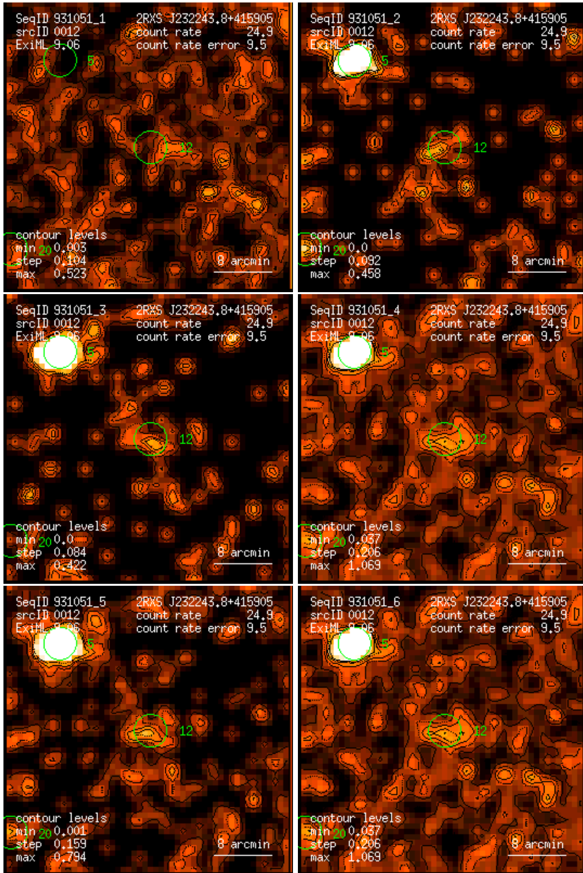
Figure 12: RASS 931051: detection 0012: band rate images, Gaussian filter: (1) PSPC channels 11 – 41, (2) 52 – 90, (3) 91 – 201, (4) 11 – 235, (5) 52 – 201, (6) 11 – 201. Broad band rates in counts/ks. Band rate contour levels in counts/ks/arcmin 2 .
