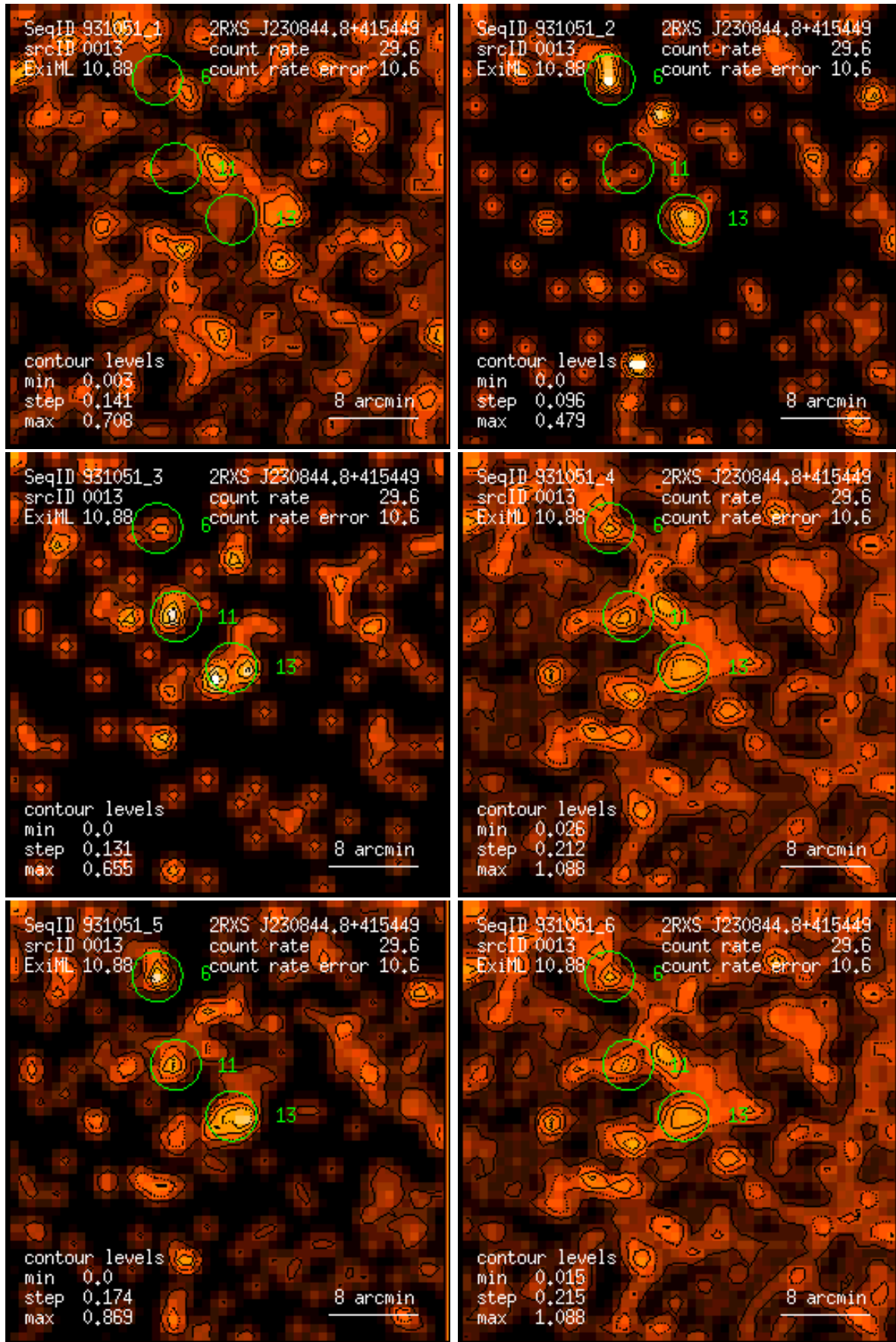
Figure 13: RASS 931051: detection 0013: band rate images, Gaussian filter: (1) PSPC channels 11 – 41, (2) 52 – 90, (3) 91 – 201, (4) 11 – 235, (5) 52 – 201, (6) 11 – 201. Broad band rates in counts/ks. Band rate contour levels in counts/ks/arcmin 2 .
