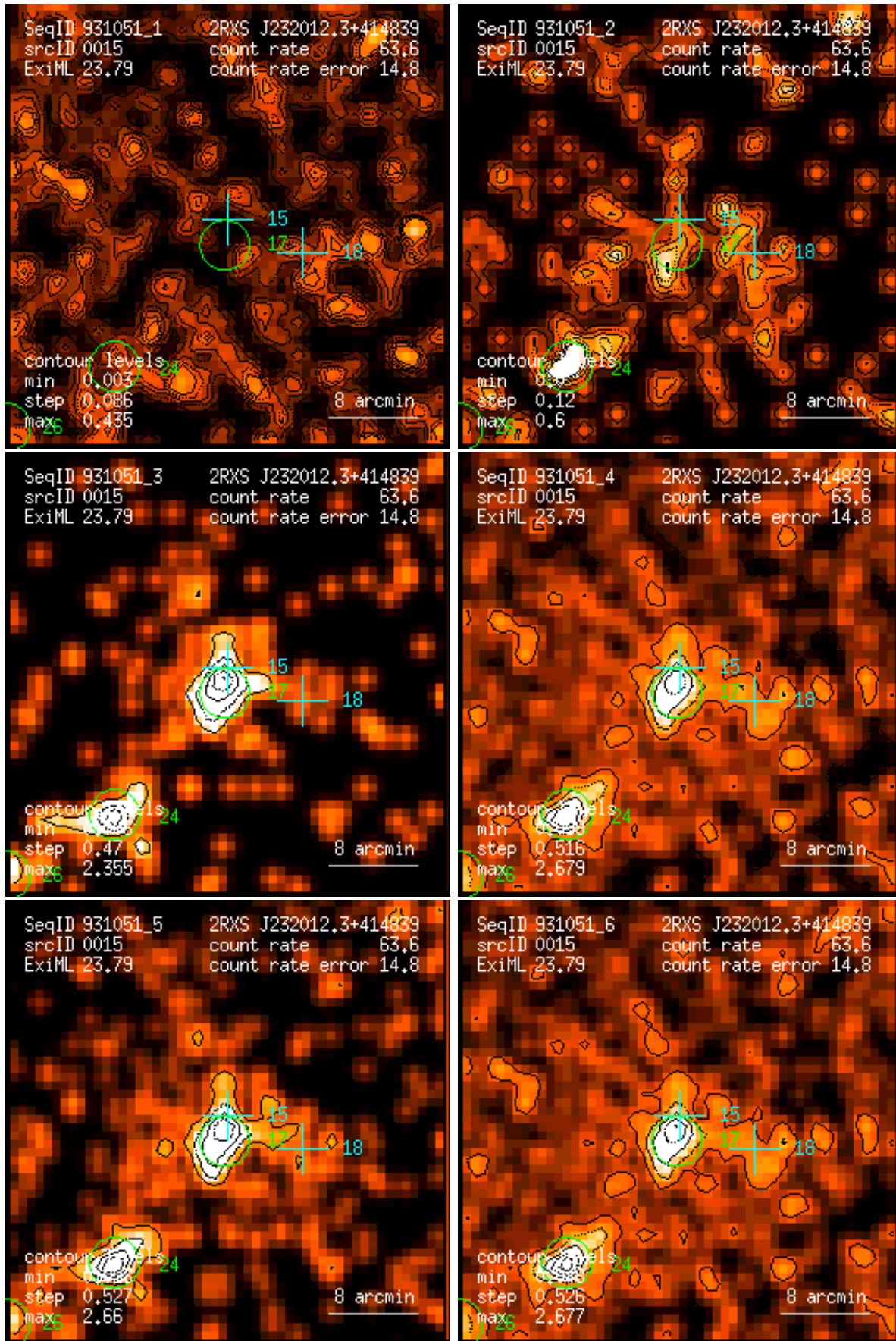
Figure 15: RASS 931051: detection 0015: band rate images, Gaussian filter: (1) PSPC channels 11 – 41, (2) 52 – 90, (3) 91 – 201, (4) 11 – 235, (5) 52 – 201, (6) 11 – 201. Broad band rates in counts/ks. Band rate contour levels in counts/ks/arcmin 2 .
