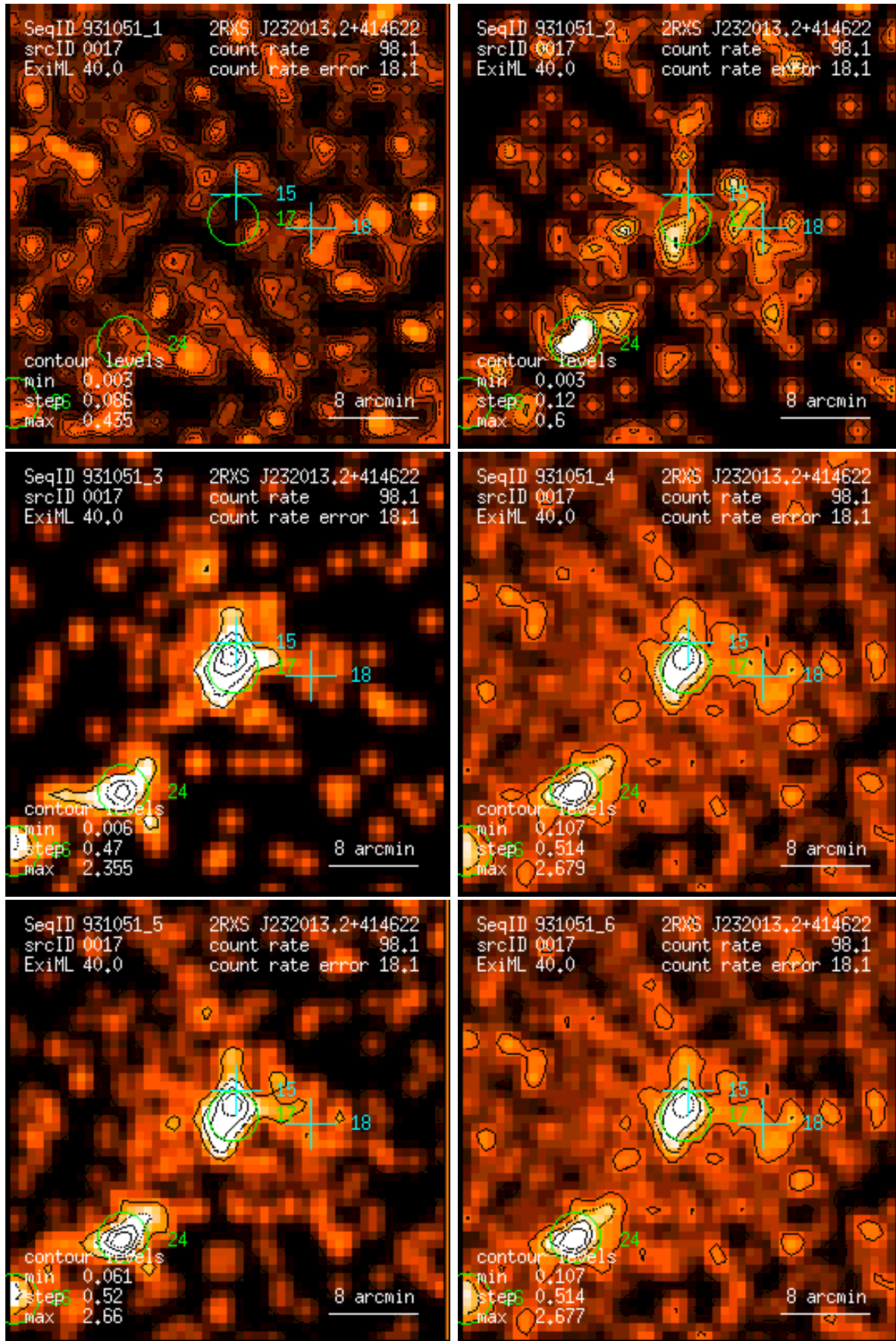
Figure 17: RASS 931051: detection 0017: band rate images, Gaussian filter: (1) PSPC channels 11 – 41, (2) 52 – 90, (3) 91 – 201, (4) 11 – 235, (5) 52 – 201, (6) 11 – 201. Broad band rates in counts/ks. Band rate contour levels in counts/ks/arcmin 2 .
