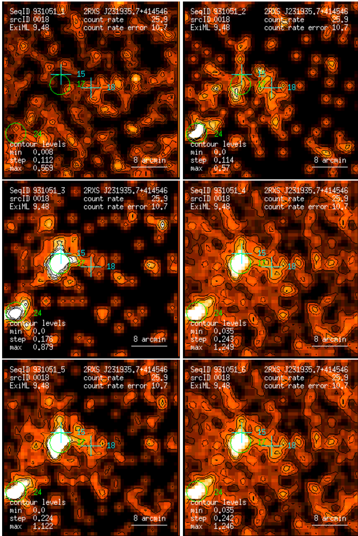
Figure 18: RASS 931051: detection 0018: band rate images, Gaussian filter: (1) PSPC channels 11 – 41, (2) 52 – 90, (3) 91 – 201, (4) 11 – 235, (5) 52 – 201, (6) 11 – 201. Broad band rates in counts/ks. Band rate contour levels in counts/ks/arcmin 2 .
