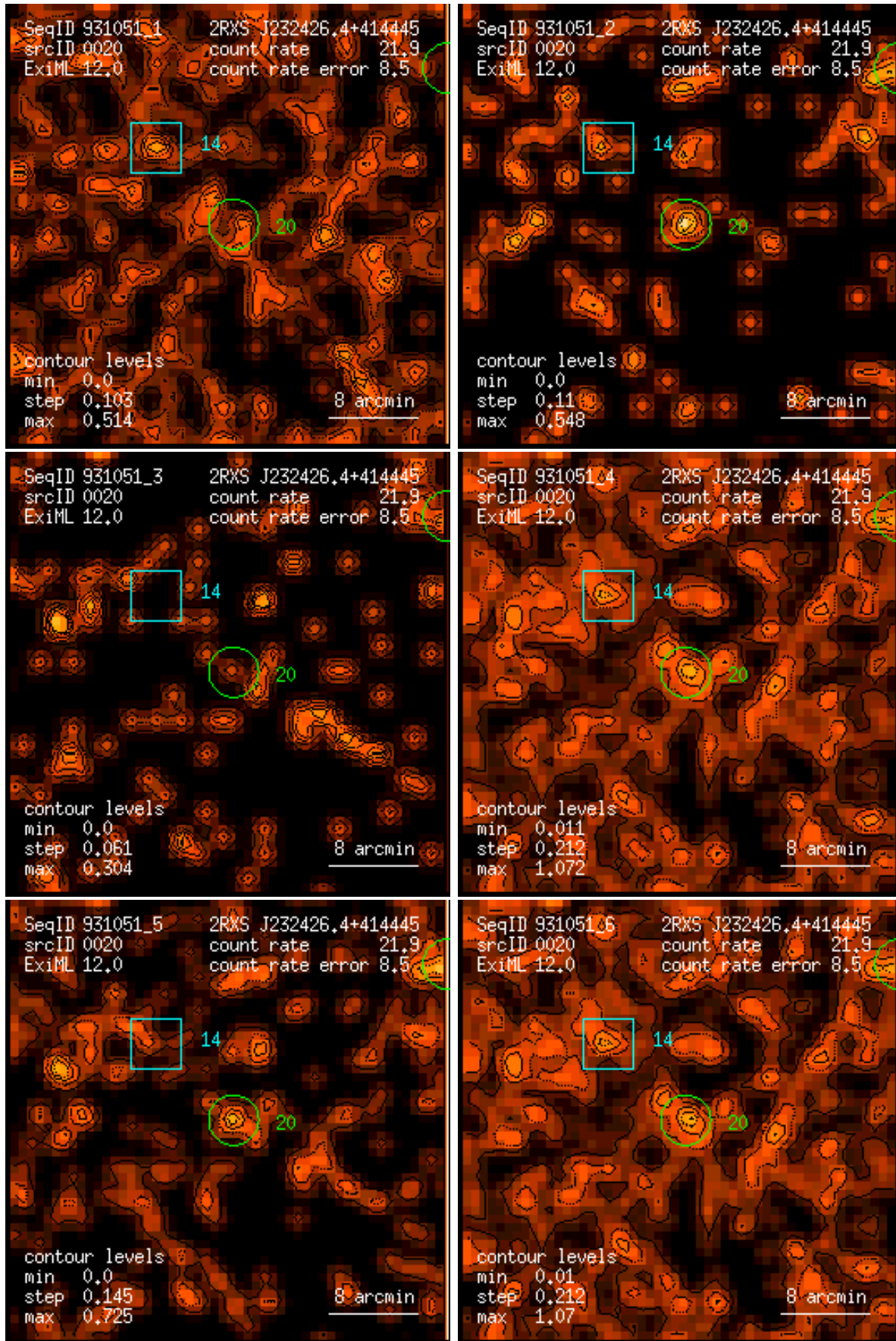
Figure 20: RASS 931051: detection 0020: band rate images, Gaussian filter: (1) PSPC channels 11 – 41, (2) 52 – 90, (3) 91 – 201, (4) 11 – 235, (5) 52 – 201, (6) 11 – 201. Broad band rates in counts/ks. Band rate contour levels in counts/ks/arcmin 2 .
