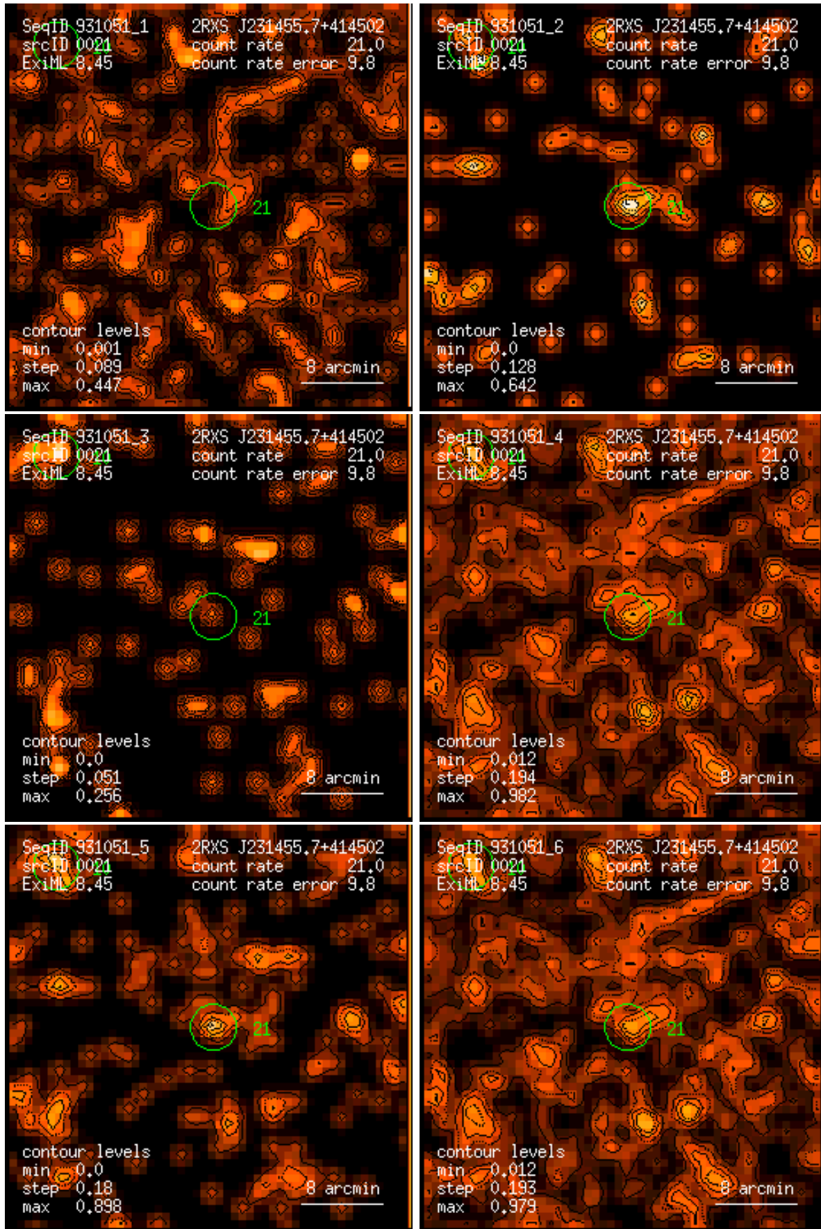
Figure 21: RASS 931051: detection 0021: band rate images, Gaussian filter: (1) PSPC channels 11 – 41, (2) 52 – 90, (3) 91 – 201, (4) 11 – 235, (5) 52 – 201, (6) 11 – 201. Broad band rates in counts/ks. Band rate contour levels in counts/ks/arcmin 2 .
