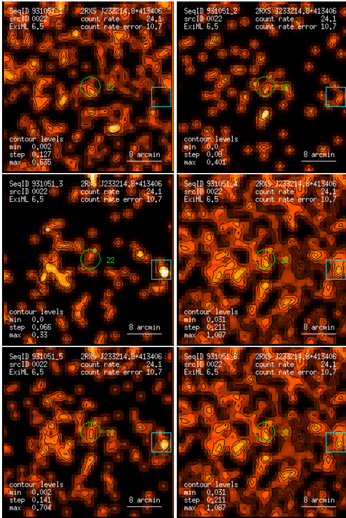
Figure 22: RASS 931051: detection 0022: band rate images, Gaussian filter: (1) PSPC channels 11 – 41, (2) 52 – 90, (3) 91 – 201, (4) 11 – 235, (5) 52 – 201, (6) 11 – 201. Broad band rates in counts/ks. Band rate contour levels in counts/ks/arcmin 2 .
