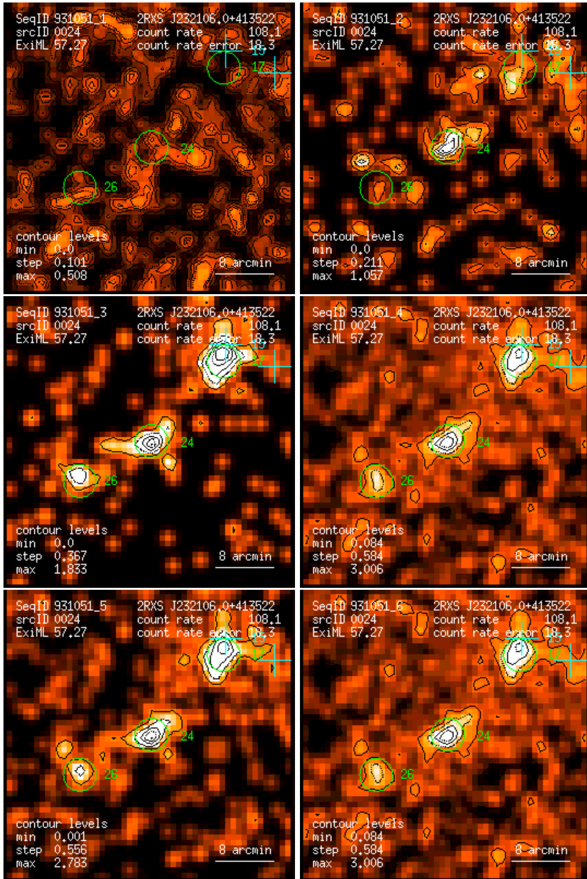
Figure 24: RASS 931051: detection 0024: band rate images, Gaussian filter: (1) PSPC channels 11 – 41, (2) 52 – 90, (3) 91 – 201, (4) 11 – 235, (5) 52 – 201, (6) 11 – 201. Broad band rates in counts/ks. Band rate contour levels in counts/ks/arcmin 2 .
