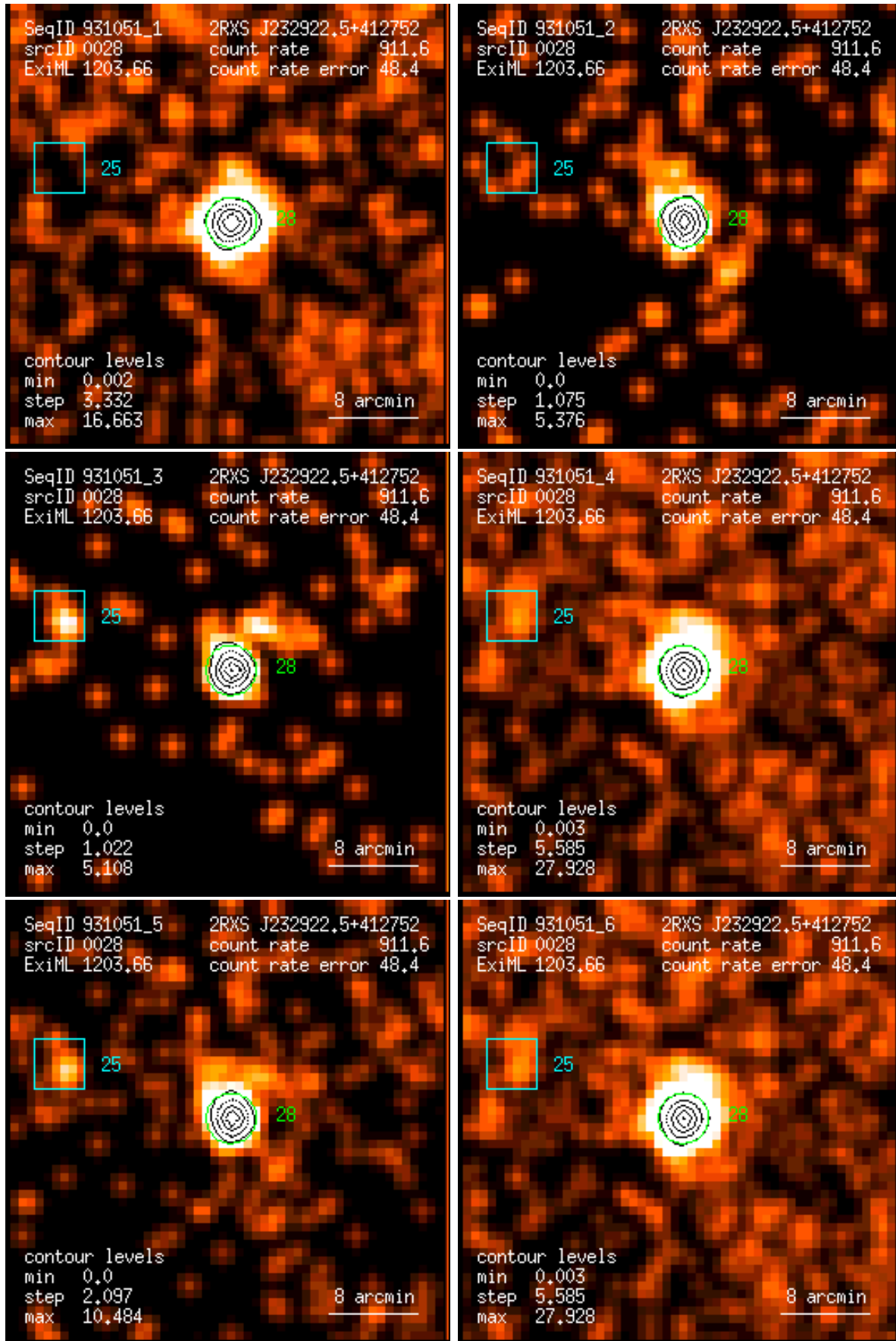
Figure 28: RASS 931051: detection 0028: band rate images, Gaussian filter: (1) PSPC channels 11 – 41, (2) 52 – 90, (3) 91 – 201, (4) 11 – 235, (5) 52 – 201, (6) 11 – 201. Broad band rates in counts/ks. Band rate contour levels in counts/ks/arcmin 2 .
