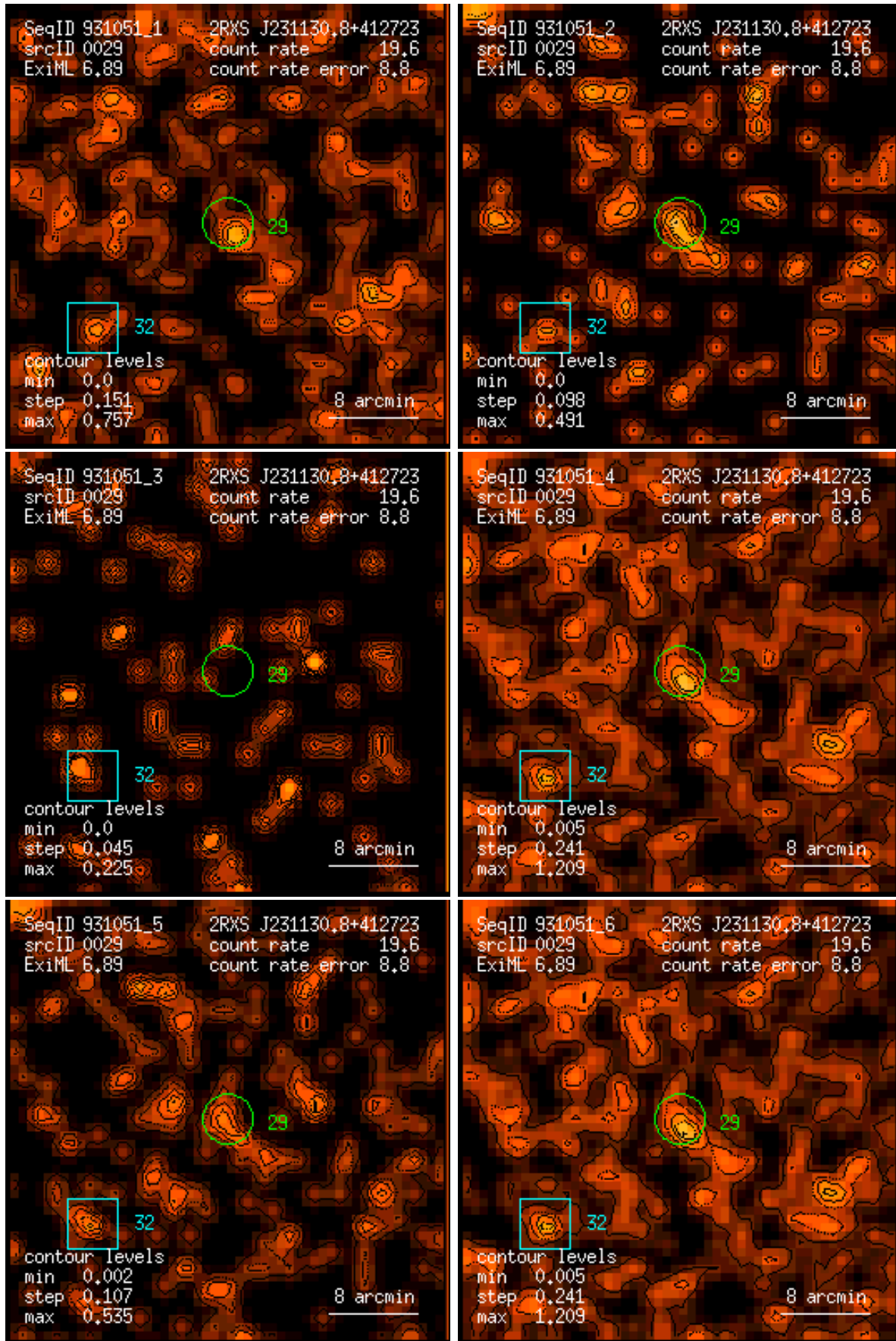
Figure 29: RASS 931051: detection 0029: band rate images, Gaussian filter: (1) PSPC channels 11 – 41, (2) 52 – 90, (3) 91 – 201, (4) 11 – 235, (5) 52 – 201, (6) 11 – 201. Broad band rates in counts/ks. Band rate contour levels in counts/ks/arcmin 2 .
