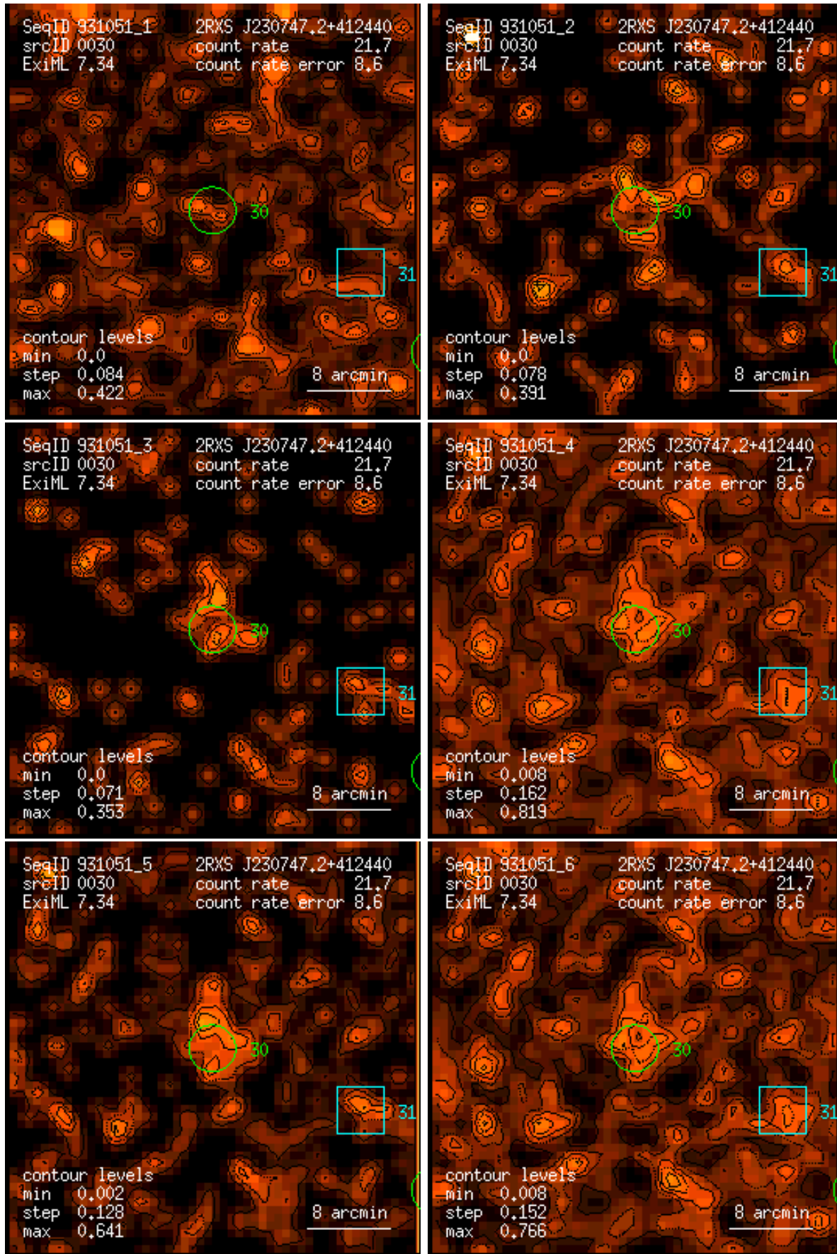
Figure 30: RASS 931051: detection 0030: band rate images, Gaussian filter: (1) PSPC channels 11 – 41, (2) 52 – 90, (3) 91 – 201, (4) 11 – 235, (5) 52 – 201, (6) 11 – 201. Broad band rates in counts/ks. Band rate contour levels in counts/ks/arcmin 2 .
