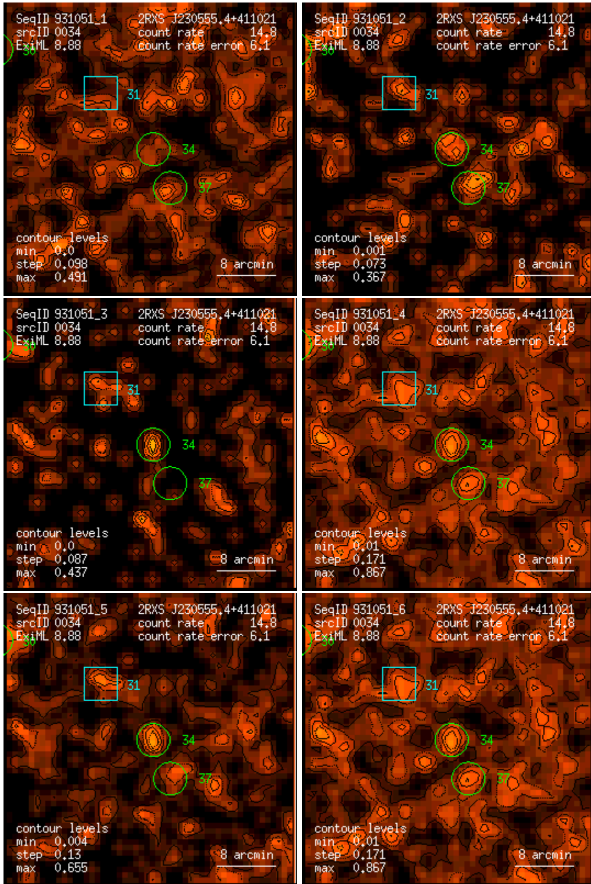
Figure 34: RASS 931051: detection 0034: band rate images, Gaussian filter: (1) PSPC channels 11 – 41, (2) 52 – 90, (3) 91 – 201, (4) 11 – 235, (5) 52 – 201, (6) 11 – 201. Broad band rates in counts/ks. Band rate contour levels in counts/ks/arcmin 2 .
