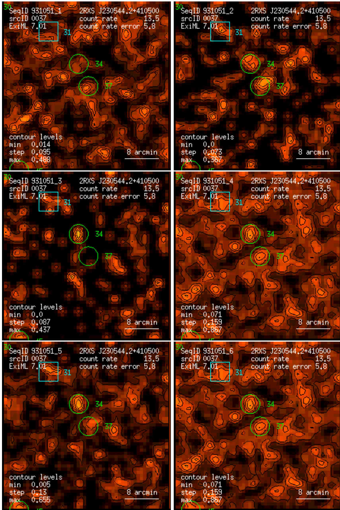
Figure 37: RASS 931051: detection 0037: band rate images, Gaussian filter: (1) PSPC channels 11 – 41, (2) 52 – 90, (3) 91 – 201, (4) 11 – 235, (5) 52 – 201, (6) 11 – 201. Broad band rates in counts/ks. Band rate contour levels in counts/ks/arcmin 2 .
