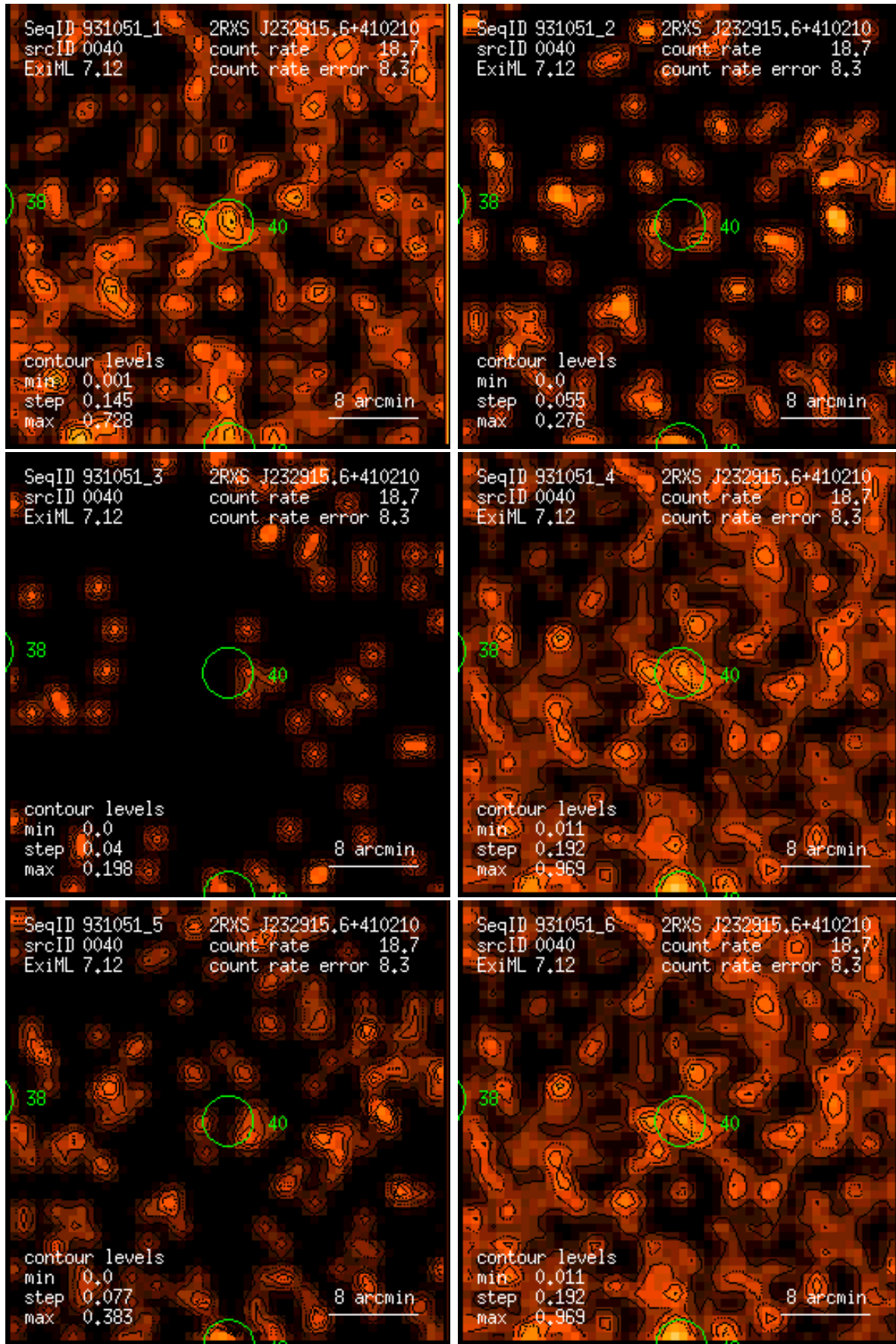
Figure 40: RASS 931051: detection 0040: band rate images, Gaussian filter: (1) PSPC channels 11 – 41, (2) 52 – 90, (3) 91 – 201, (4) 11 – 235, (5) 52 – 201, (6) 11 – 201. Broad band rates in counts/ks. Band rate contour levels in counts/ks/arcmin 2 .
