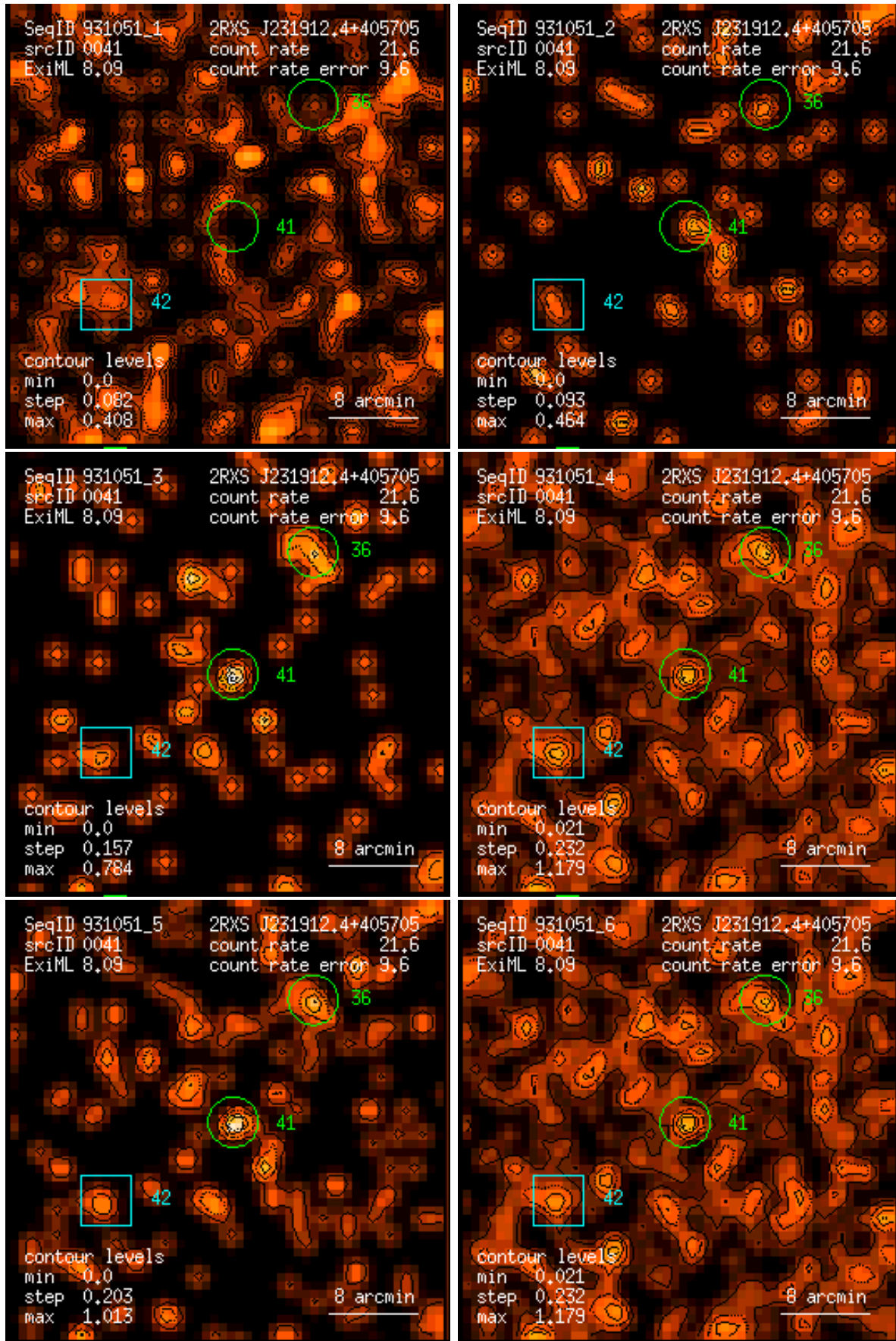
Figure 41: RASS 931051: detection 0041: band rate images, Gaussian filter: (1) PSPC channels 11 – 41, (2) 52 – 90, (3) 91 – 201, (4) 11 – 235, (5) 52 – 201, (6) 11 – 201. Broad band rates in counts/ks. Band rate contour levels in counts/ks/arcmin 2 .
