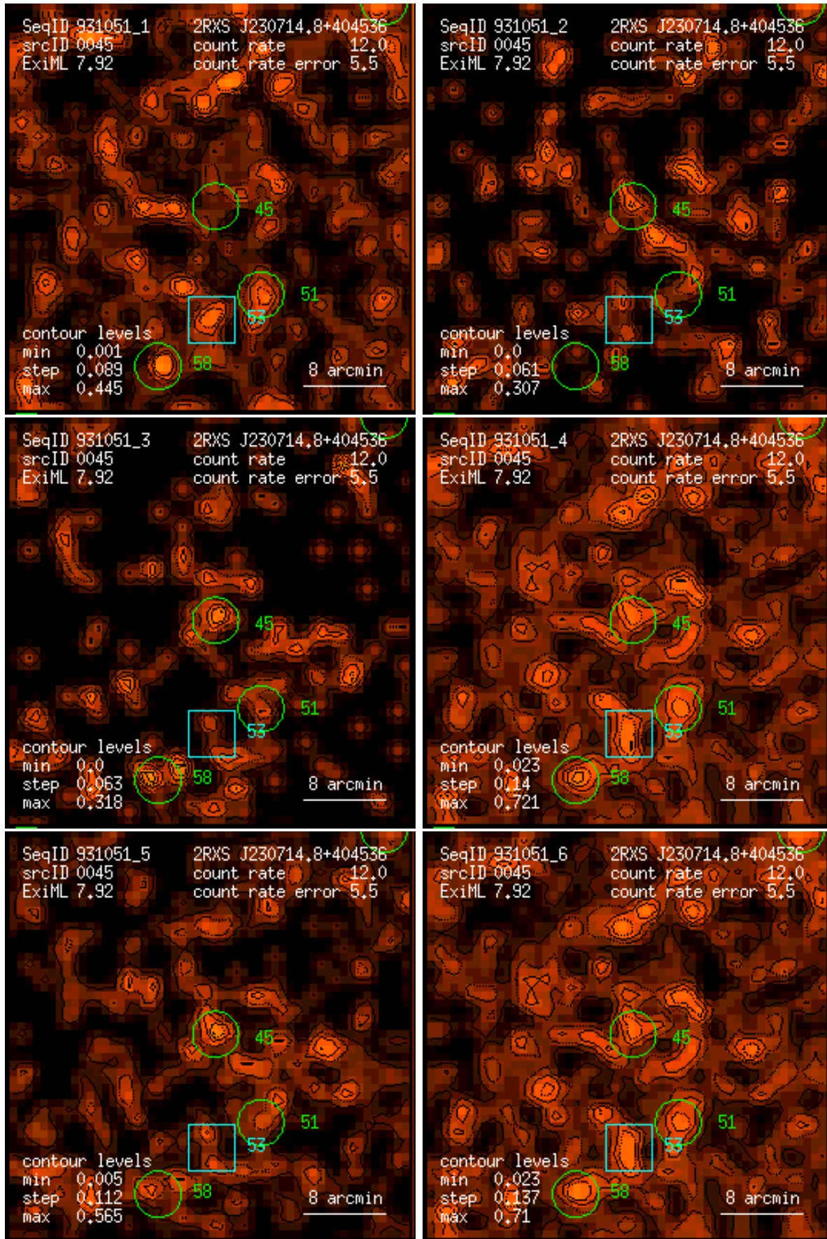
Figure 45: RASS 931051: detection 0045: band rate images, Gaussian filter: (1) PSPC channels 11 – 41, (2) 52 – 90, (3) 91 – 201, (4) 11 – 235, (5) 52 – 201, (6) 11 – 201. Broad band rates in counts/ks. Band rate contour levels in counts/ks/arcmin 2 .
