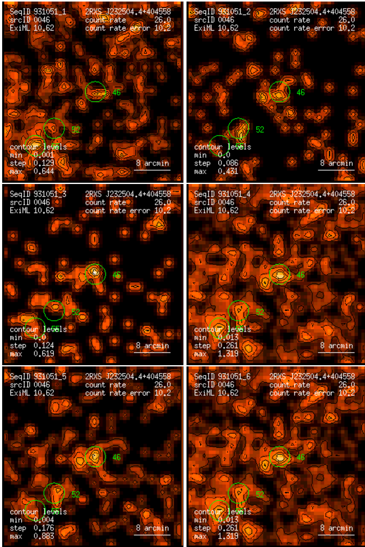
Figure 46: RASS 931051: detection 0046: band rate images, Gaussian filter: (1) PSPC channels 11 – 41, (2) 52 – 90, (3) 91 – 201, (4) 11 – 235, (5) 52 – 201, (6) 11 – 201. Broad band rates in counts/ks. Band rate contour levels in counts/ks/arcmin 2 .
