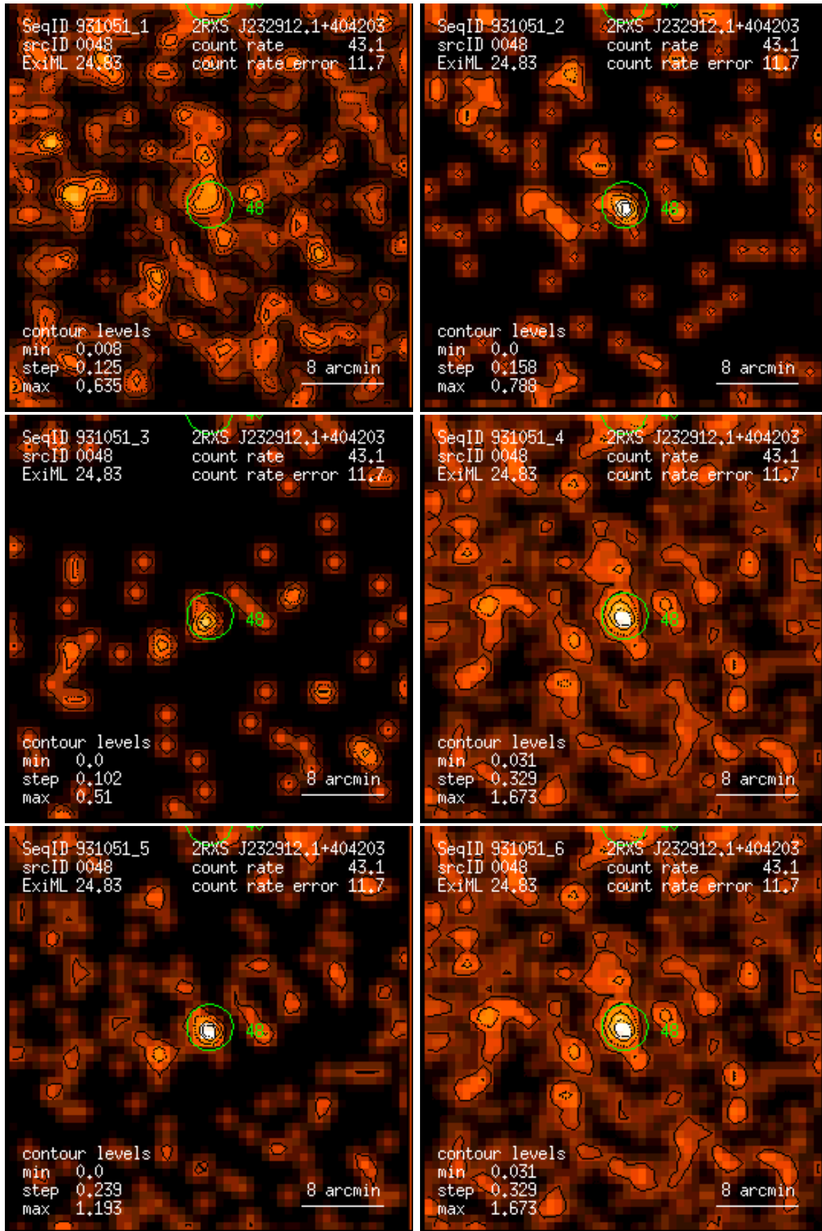
Figure 48: RASS 931051: detection 0048: band rate images, Gaussian filter: (1) PSPC channels 11 – 41, (2) 52 – 90, (3) 91 – 201, (4) 11 – 235, (5) 52 – 201, (6) 11 – 201. Broad band rates in counts/ks. Band rate contour levels in counts/ks/arcmin 2 .
