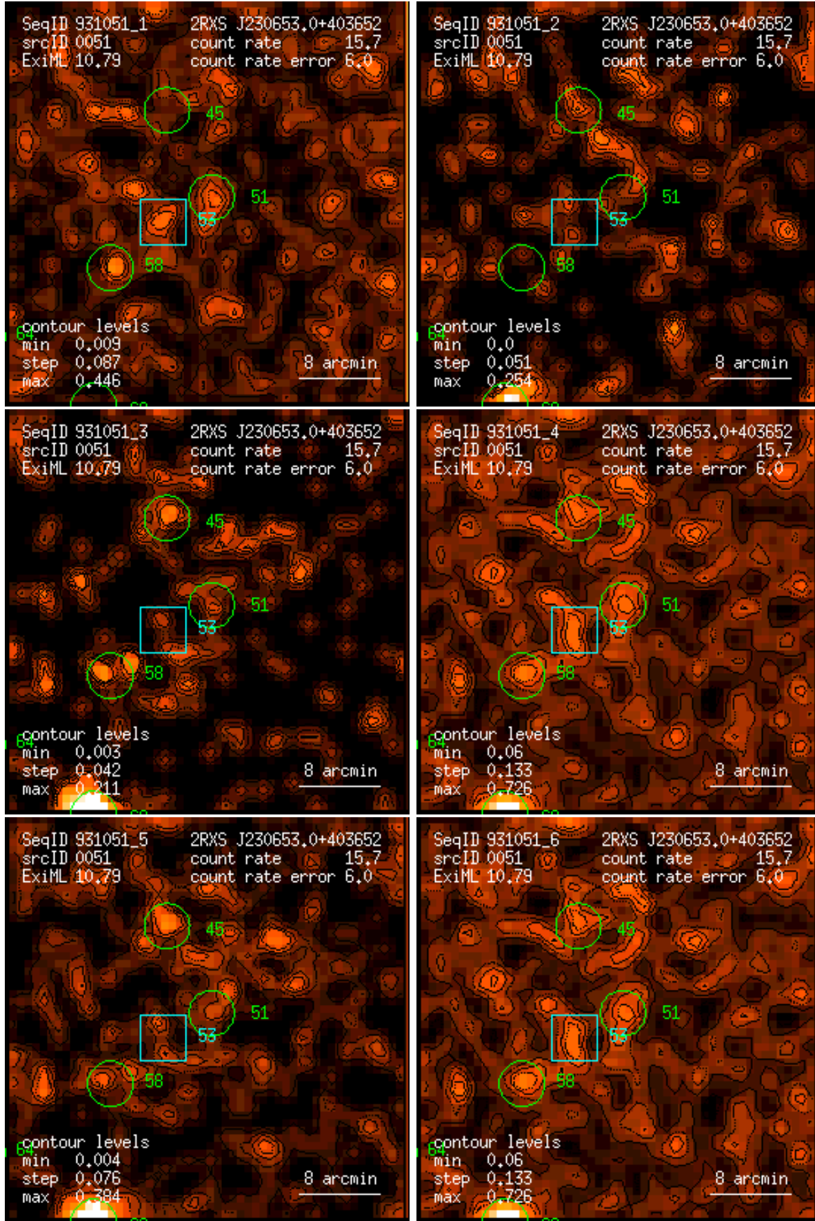
Figure 51: RASS 931051: detection 0051: band rate images, Gaussian filter: (1) PSPC channels 11 – 41, (2) 52 – 90, (3) 91 – 201, (4) 11 – 235, (5) 52 – 201, (6) 11 – 201. Broad band rates in counts/ks. Band rate contour levels in counts/ks/arcmin 2 .
