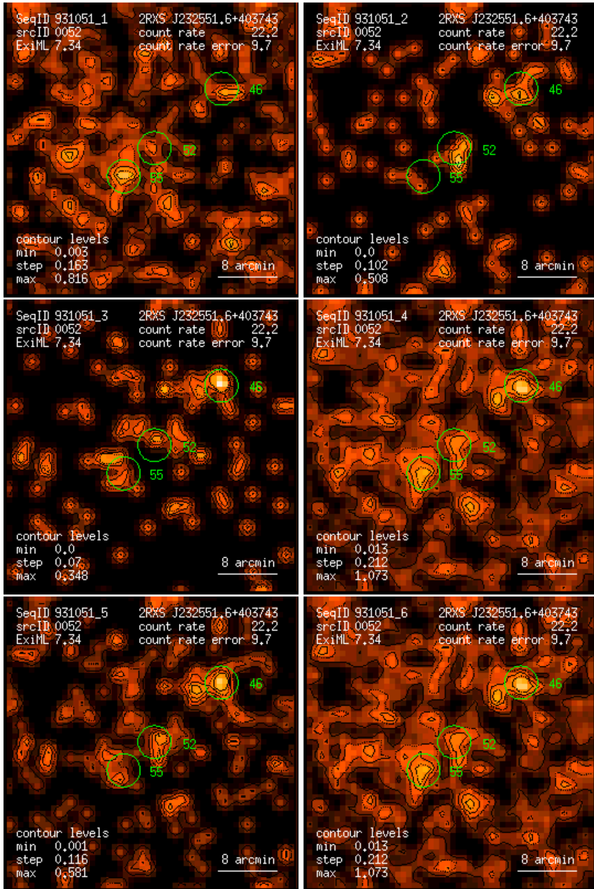
Figure 52: RASS 931051: detection 0052: band rate images, Gaussian filter: (1) PSPC channels 11 – 41, (2) 52 – 90, (3) 91 – 201, (4) 11 – 235, (5) 52 – 201, (6) 11 – 201. Broad band rates in counts/ks. Band rate contour levels in counts/ks/arcmin 2 .
