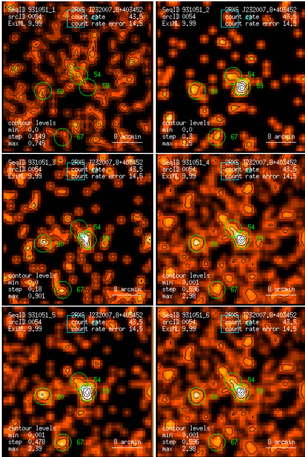
Figure 54: RASS 931051: detection 0054: band rate images, Gaussian filter: (1) PSPC channels 11 – 41, (2) 52 – 90, (3) 91 – 201, (4) 11 – 235, (5) 52 – 201, (6) 11 – 201. Broad band rates in counts/ks. Band rate contour levels in counts/ks/arcmin 2 .
