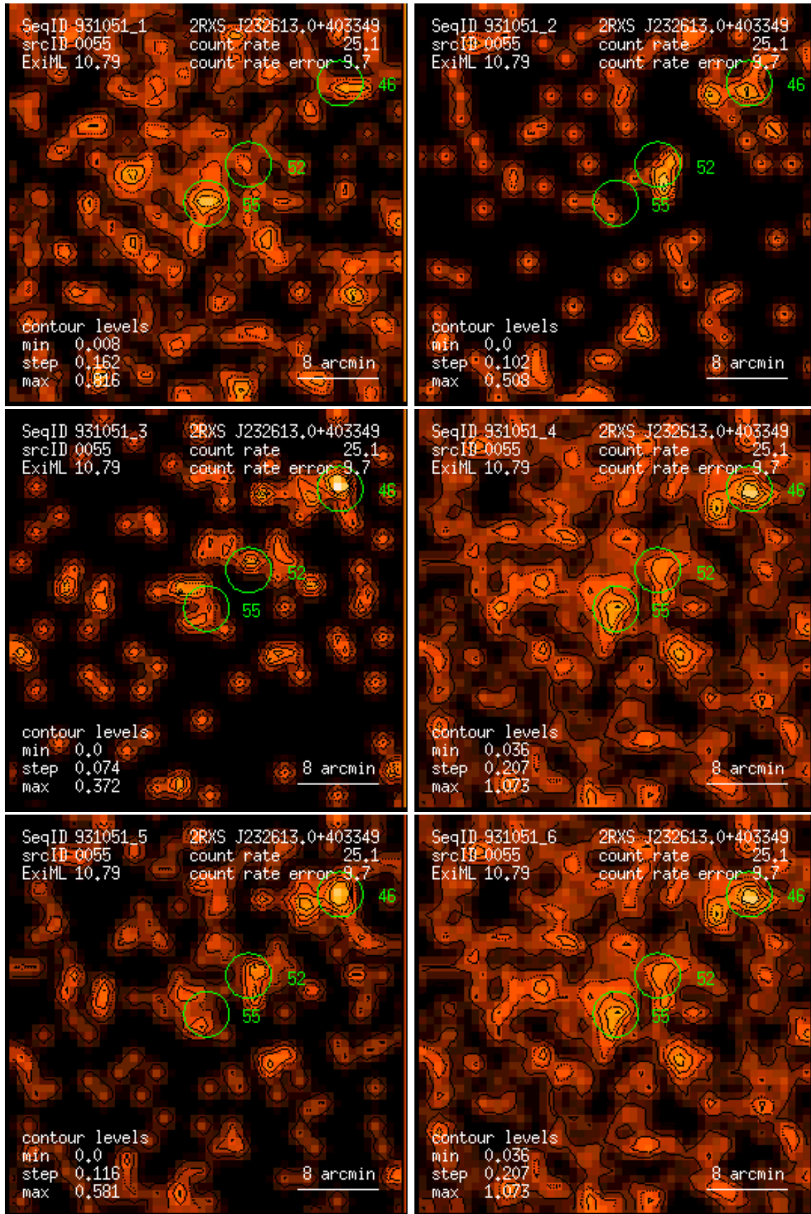
Figure 55: RASS 931051: detection 0055: band rate images, Gaussian filter: (1) PSPC channels 11 – 41, (2) 52 – 90, (3) 91 – 201, (4) 11 – 235, (5) 52 – 201, (6) 11 – 201. Broad band rates in counts/ks. Band rate contour levels in counts/ks/arcmin 2 .
