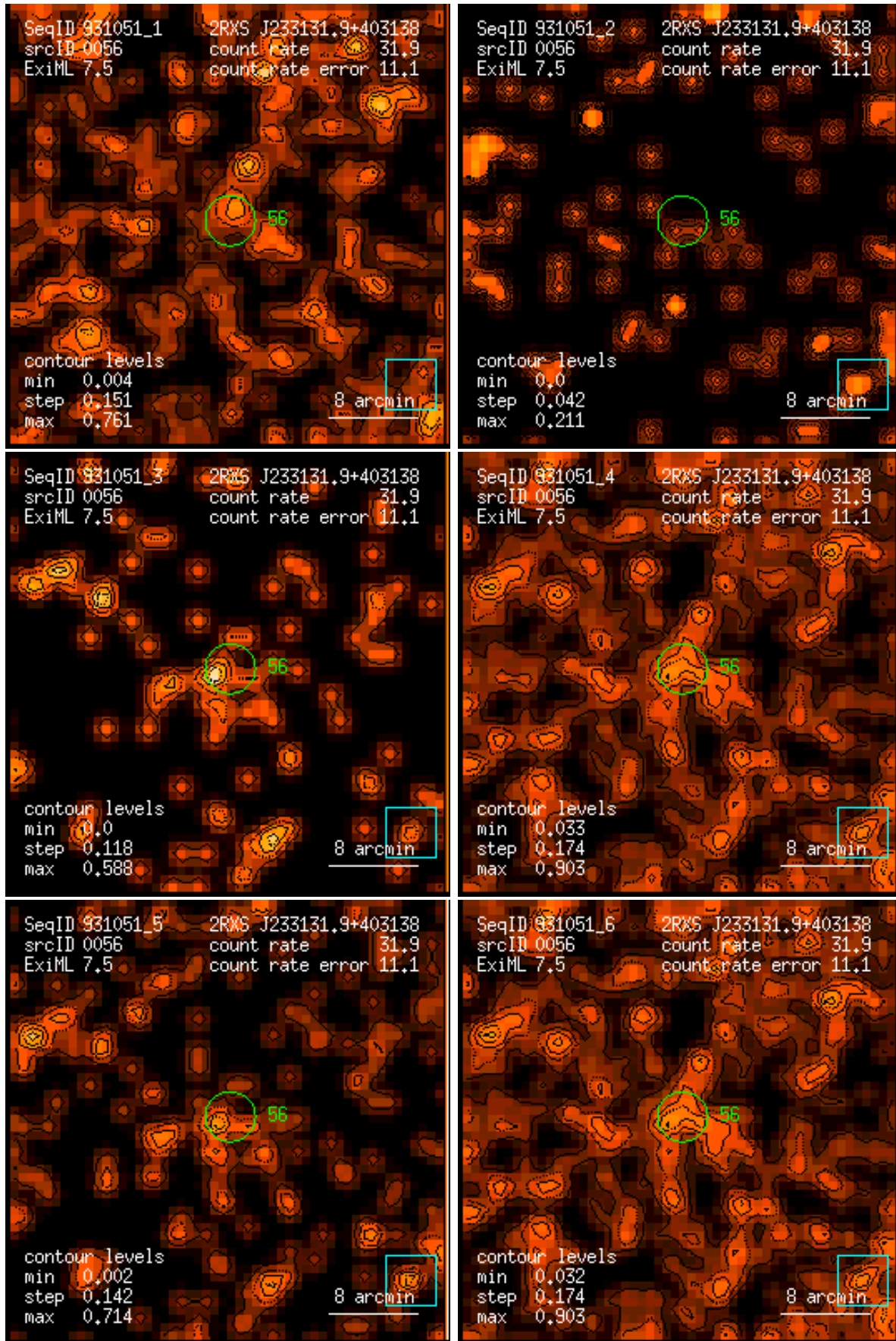
Figure 56: RASS 931051: detection 0056: band rate images, Gaussian filter: (1) PSPC channels 11 – 41, (2) 52 – 90, (3) 91 – 201, (4) 11 – 235, (5) 52 – 201, (6) 11 – 201. Broad band rates in counts/ks. Band rate contour levels in counts/ks/arcmin 2 .
