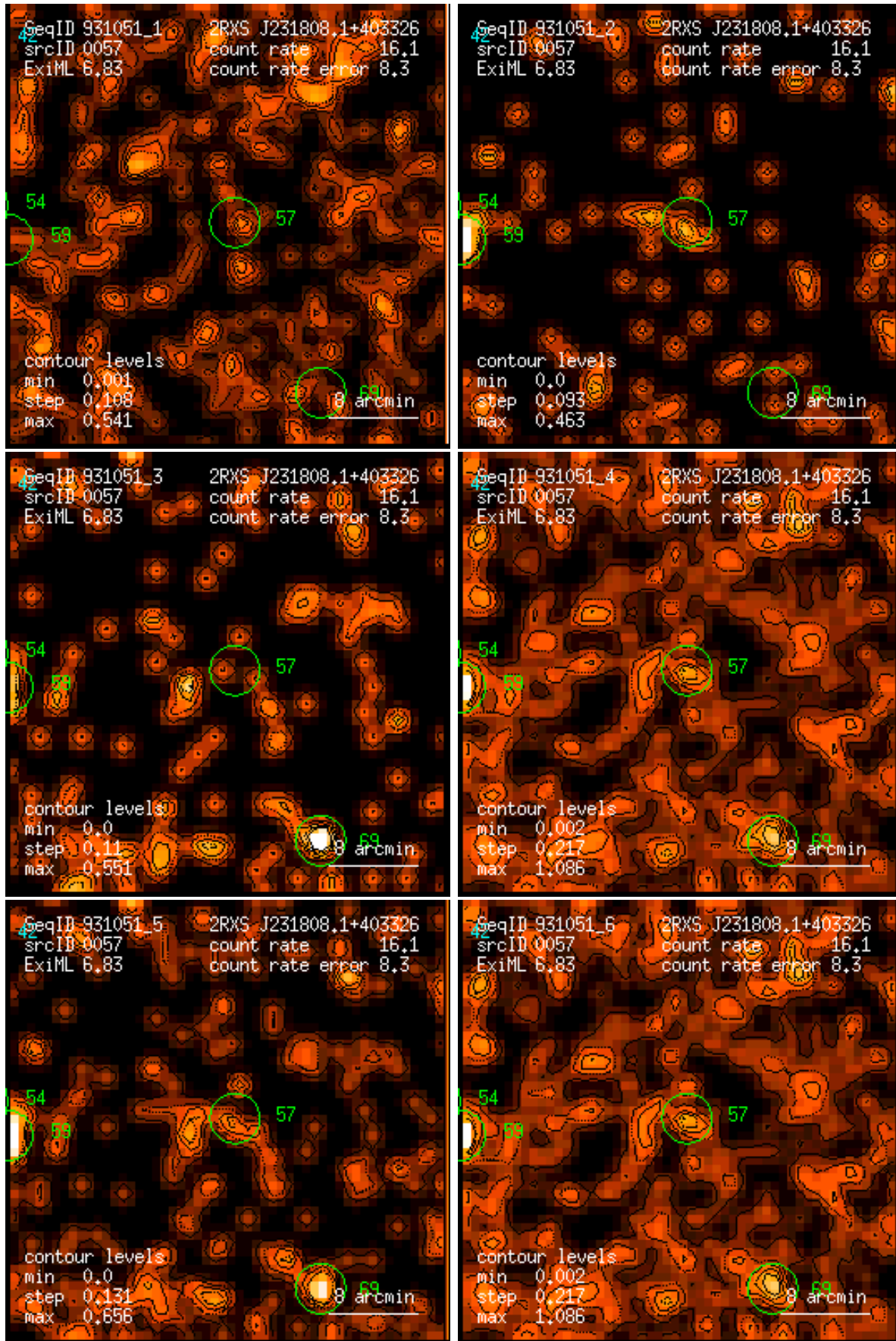
Figure 57: RASS 931051: detection 0057: band rate images, Gaussian filter: (1) PSPC channels 11 – 41, (2) 52 – 90, (3) 91 – 201, (4) 11 – 235, (5) 52 – 201, (6) 11 – 201. Broad band rates in counts/ks. Band rate contour levels in counts/ks/arcmin 2 .
