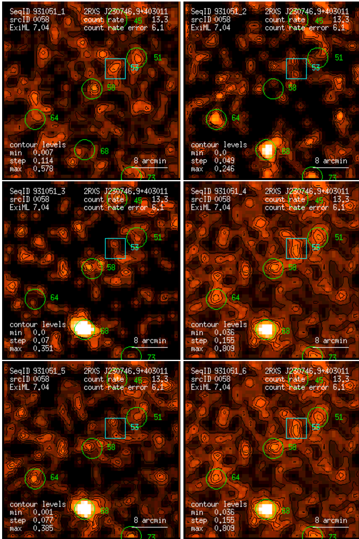
Figure 58: RASS 931051: detection 0058: band rate images, Gaussian filter: (1) PSPC channels 11 – 41, (2) 52 – 90, (3) 91 – 201, (4) 11 – 235, (5) 52 – 201, (6) 11 – 201. Broad band rates in counts/ks. Band rate contour levels in counts/ks/arcmin 2 .
