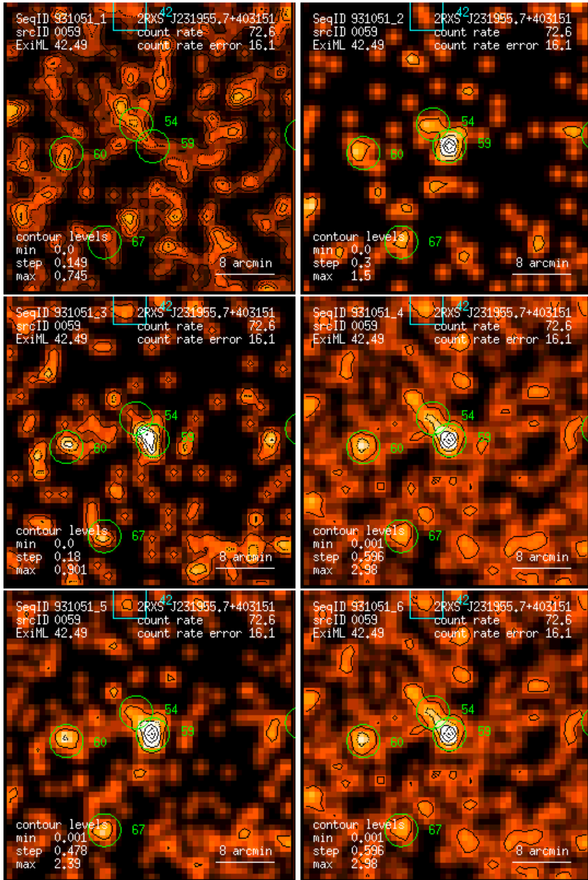
Figure 59: RASS 931051: detection 0059: band rate images, Gaussian filter: (1) PSPC channels 11 – 41, (2) 52 – 90, (3) 91 – 201, (4) 11 – 235, (5) 52 – 201, (6) 11 – 201. Broad band rates in counts/ks. Band rate contour levels in counts/ks/arcmin 2 .
