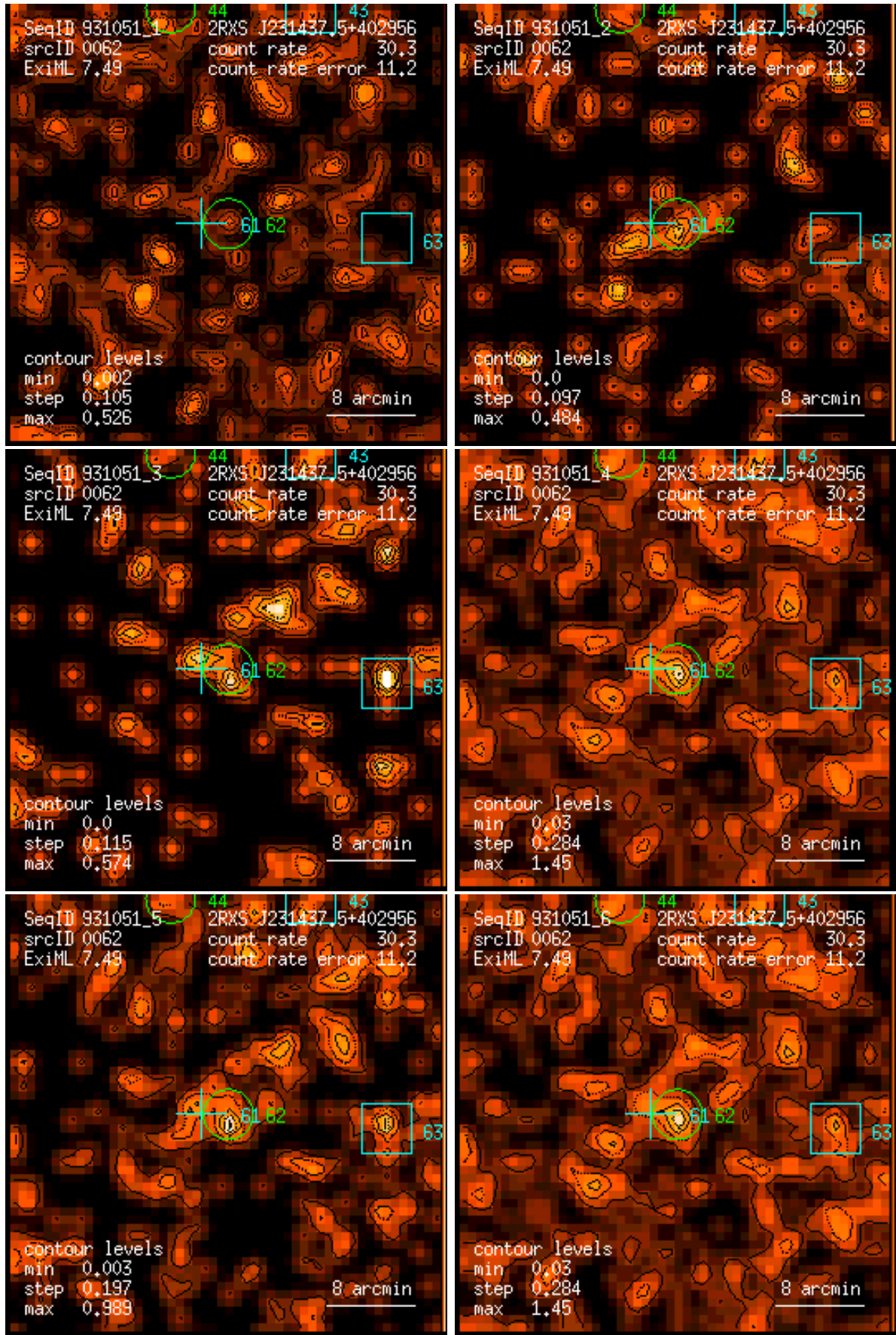
Figure 62: RASS 931051: detection 0062: band rate images, Gaussian filter: (1) PSPC channels 11 – 41, (2) 52 – 90, (3) 91 – 201, (4) 11 – 235, (5) 52 – 201, (6) 11 – 201. Broad band rates in counts/ks. Band rate contour levels in counts/ks/arcmin 2 .
