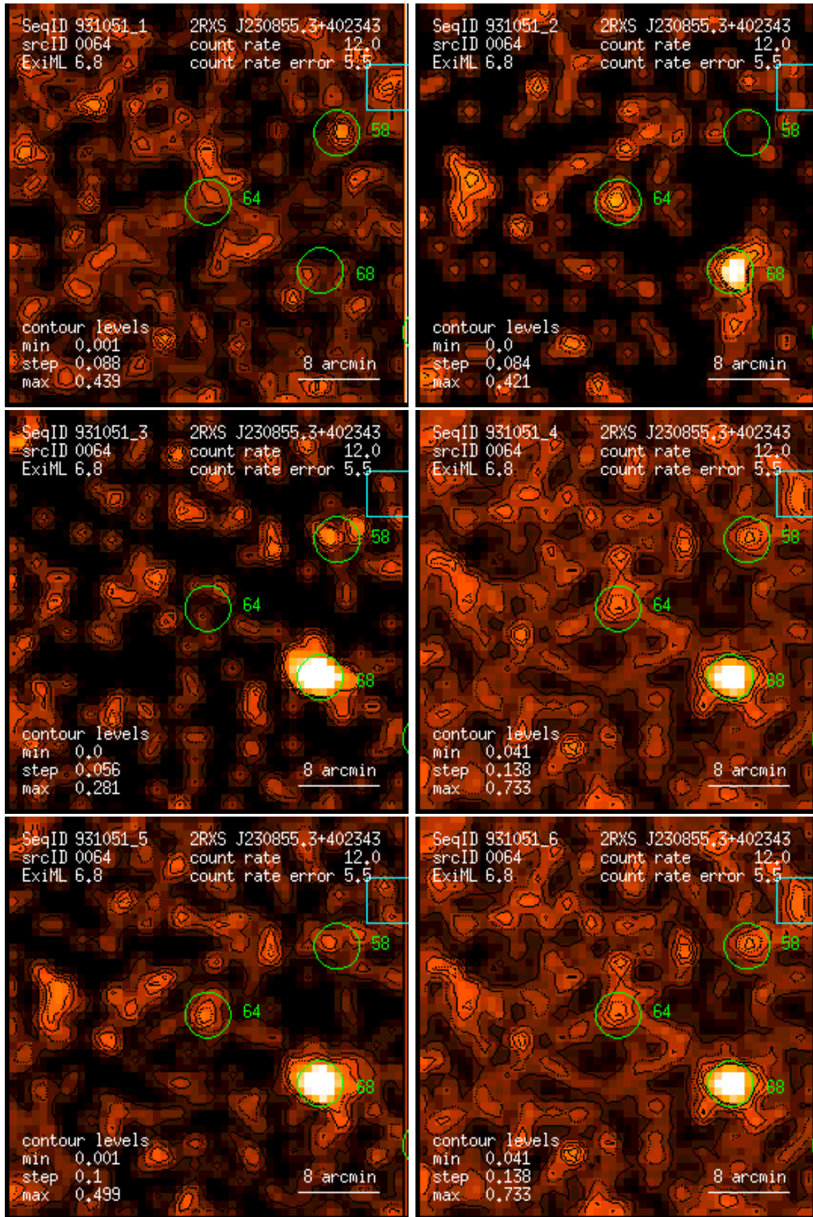
Figure 64: RASS 931051: detection 0064: band rate images, Gaussian filter: (1) PSPC channels 11 – 41, (2) 52 – 90, (3) 91 – 201, (4) 11 – 235, (5) 52 – 201, (6) 11 – 201. Broad band rates in counts/ks. Band rate contour levels in counts/ks/arcmin 2 .
