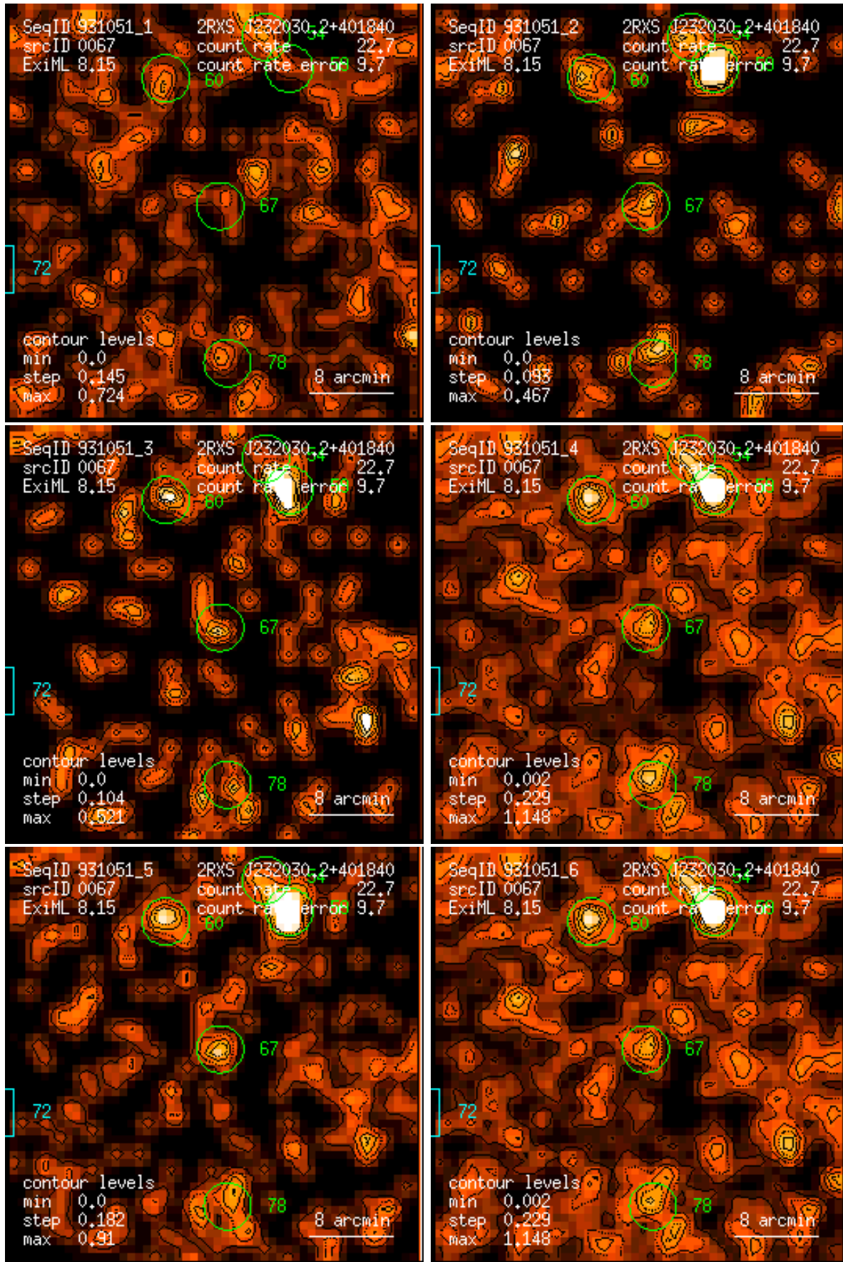
Figure 67: RASS 931051: detection 0067: band rate images, Gaussian filter: (1) PSPC channels 11 – 41, (2) 52 – 90, (3) 91 – 201, (4) 11 – 235, (5) 52 – 201, (6) 11 – 201. Broad band rates in counts/ks. Band rate contour levels in counts/ks/arcmin 2 .
