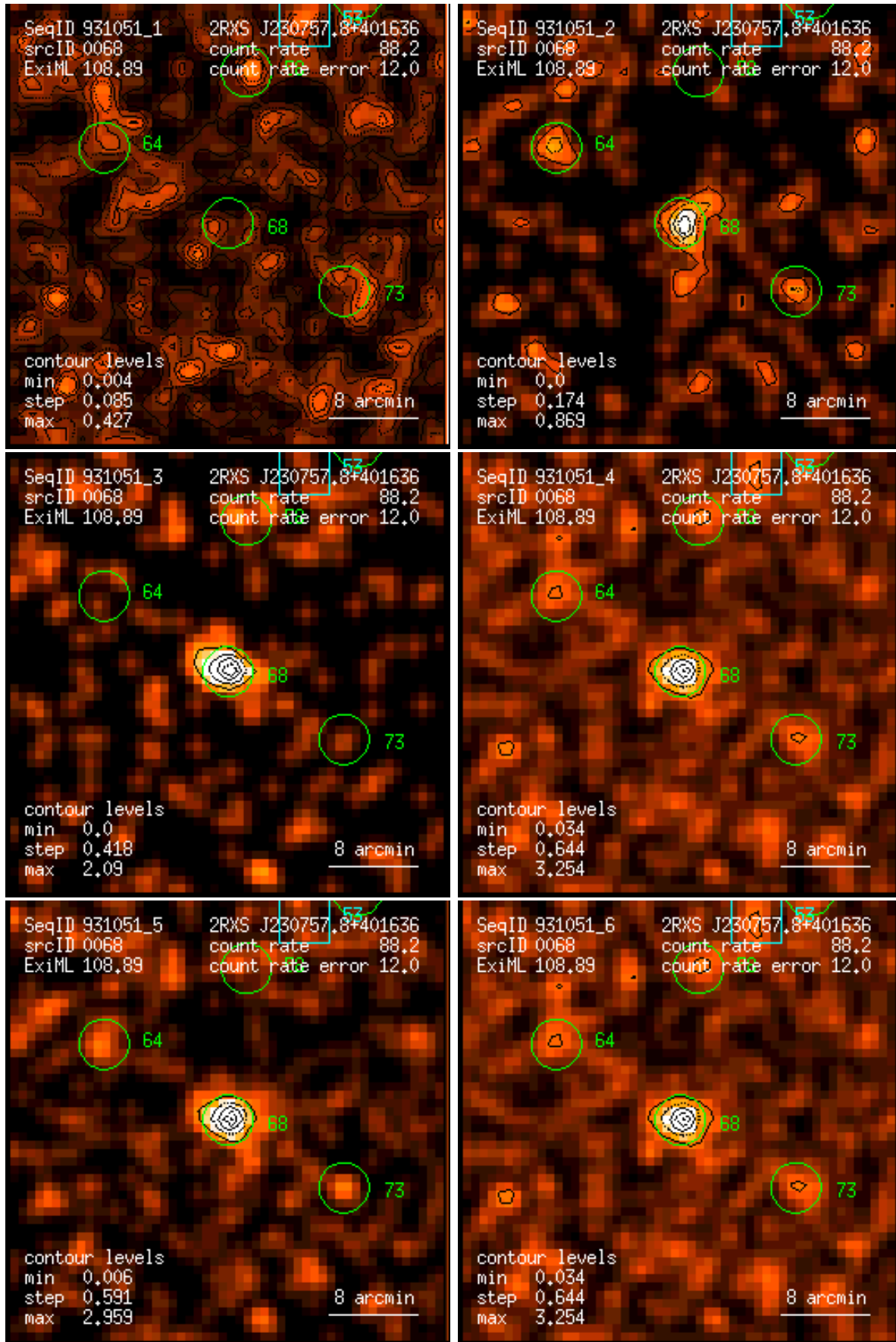
Figure 68: RASS 931051: detection 0068: band rate images, Gaussian filter: (1) PSPC channels 11 – 41, (2) 52 – 90, (3) 91 – 201, (4) 11 – 235, (5) 52 – 201, (6) 11 – 201. Broad band rates in counts/ks. Band rate contour levels in counts/ks/arcmin 2 .
