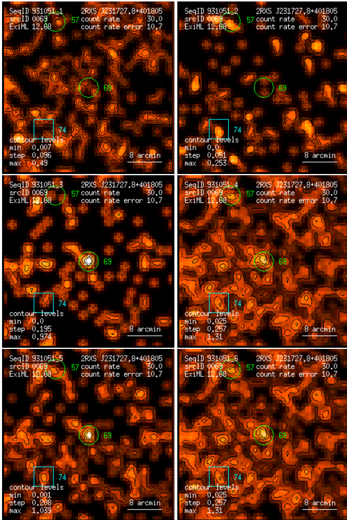
Figure 69: RASS 931051: detection 0069: band rate images, Gaussian filter: (1) PSPC channels 11 – 41, (2) 52 – 90, (3) 91 – 201, (4) 11 – 235, (5) 52 – 201, (6) 11 – 201. Broad band rates in counts/ks. Band rate contour levels in counts/ks/arcmin 2 .
