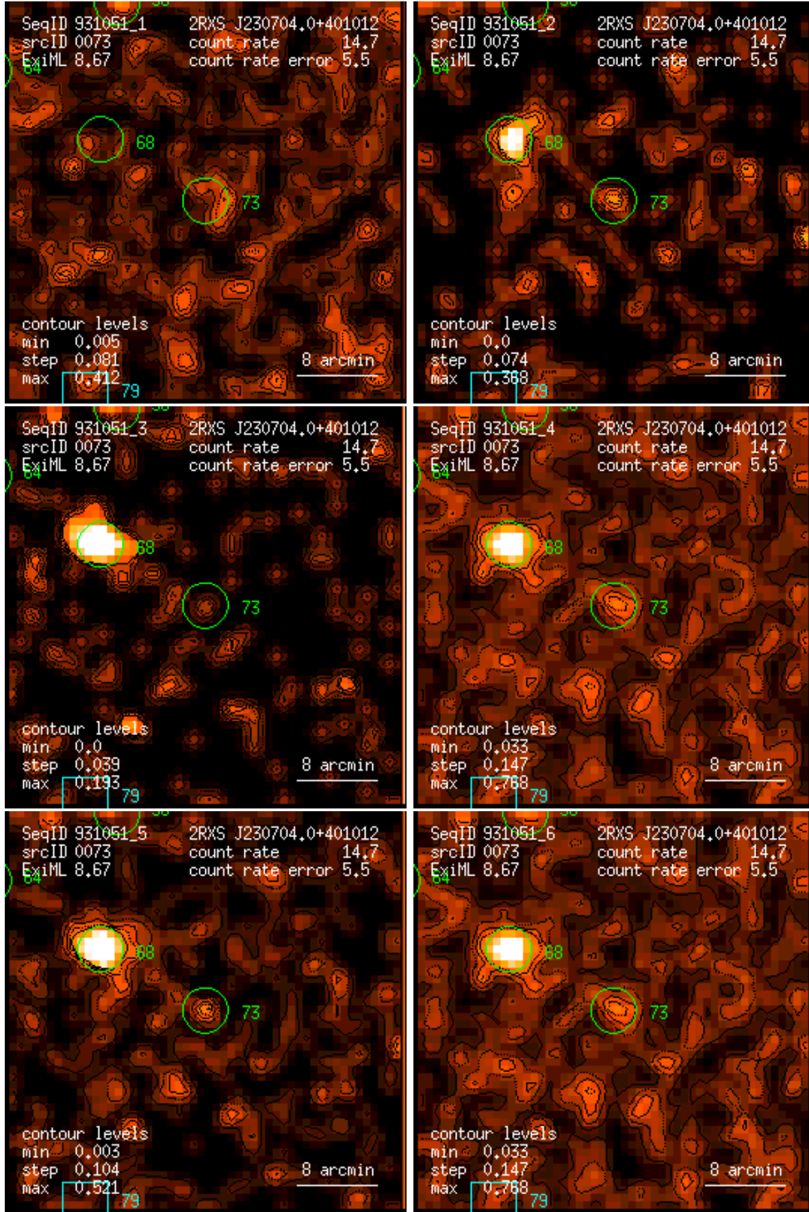
Figure 73: RASS 931051: detection 0073: band rate images, Gaussian filter: (1) PSPPC channels 11 – 41, (2) 52 – 90, (3) 91 – 201, (4) 11 – 235, (5) 52 – 201, (6) 11 – 201. Broad band rates in counts/ks. Band rate contour levels in counts/ks/arcmin 2 .
